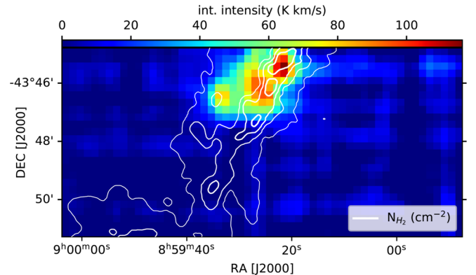
Figure 3. The integrated intensity map of [O I] at 63 \mu\text{m} from -20 to 20 km s ^{-1} , with the white contours indicating the column density N_{\text{H}_2} at (1, 2, 4, 8) \times 10^{22} cm ^{-2} .
