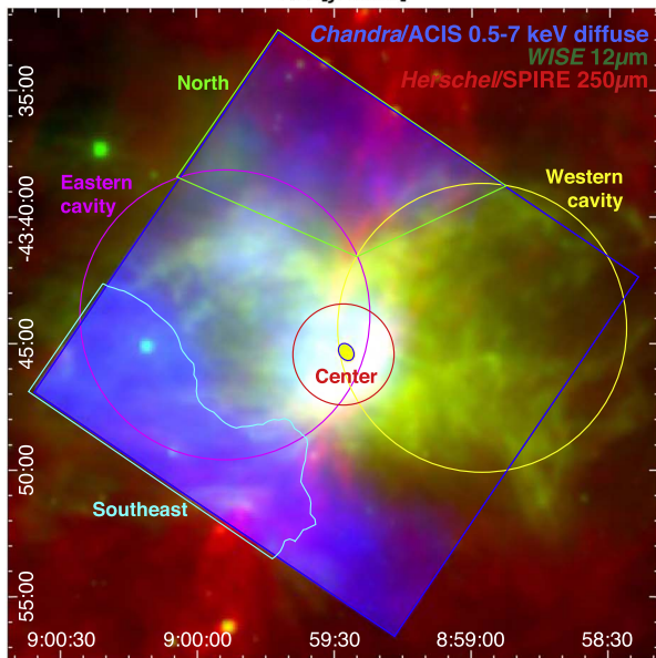
Figure 14. Top: diffuse X-ray emission observed with the ACIS instrument on Chandra. The white contours show the 70\ \mu\text{m} emission of RCW 36 from Figure 1 starting at 10^{-1.5}\ \text{Jy pixel}^{-1} with increments of 0.5 in the exponent. The brightest Chandra emission is centered on the O stars of the cluster, which are indicated by the black cross. In the cavities, there is diffuse emission detected that is significantly weaker than extended emission outside the cavities (outlined by the 70\ \mu\text{m} emission). The diffuse emission outside the cavities likely is the result of hot plasma leaking out of the H II region, which fits with the observed physical connection to the emission inside the H II region and the fact that the hot plasma fitting blindly converged to very similar properties for the different regions. Two locations where this physical connection is seen are indicated with the red lines. The red box indicates the outline of the currently observed [C II] map. Bottom: a smoothed image of Chandra/ACIS diffuse X-ray emission in the context of WISE and Herschel images. The five regions used to extract diffuse X-ray spectra are overlaid. The small blue ellipse at field center marks a region excluded from the “Center” diffuse X-ray spectrum because it is dominated by emission from unresolved young stars at the center of the cluster. See Appendix D for details of the X-ray spectral fitting.
