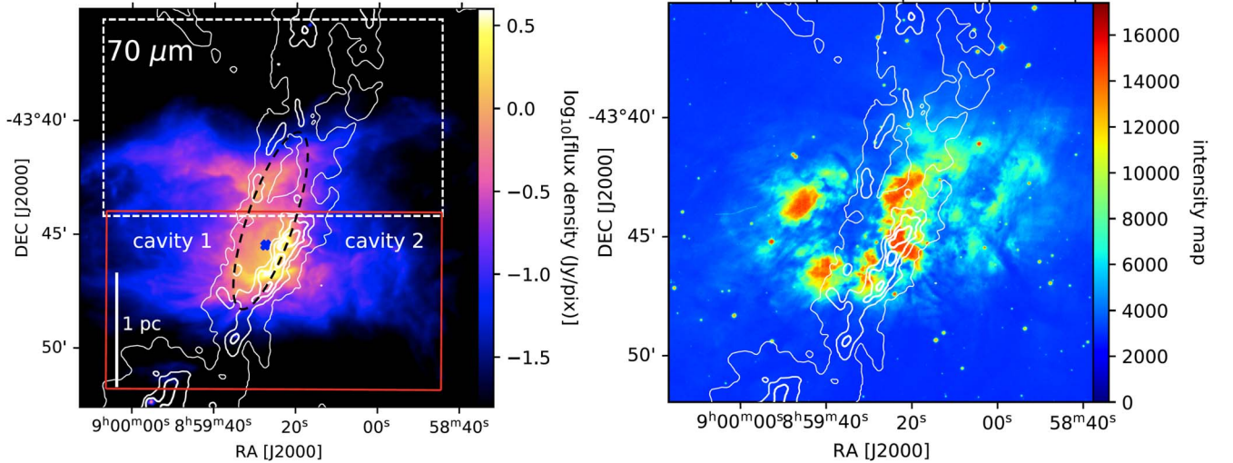
Figure 1. Left: the Herschel 70\ \mu\text{m} map of RCW 36 (Minier et al. 2013). The red box outlines the region that was already observed for the FEEDBACK program, and the dashed white box shows the area that will be mapped. The blue crosses mark the location of the two O-star candidates. Note that the close proximity of the two O-star candidates does not allow us to distinguish them clearly in this figure. The black dashed ellipse indicates the location of the central molecular ring, first reported by Minier et al. (2013). The Herschel 70\ \mu\text{m} map also traces the limb-brightened shells at the cavity walls. The white contours indicate the Herschel column density at N_{\text{H}_2} = (1, 2, 4, 8) \times 10^{22}\ \text{cm}^{-2} determined using the method presented in Palmeirim et al. (2013). Right: \text{H}\alpha intensity map toward RCW 36 from the SuperCOSMOS \text{H}\alpha Survey. The intensity units of the map are not calibrated to a specific unit and are only relative (Hamblly et al. 2001; Parker et al. 2005). The white contours again indicate the Herschel column density.
