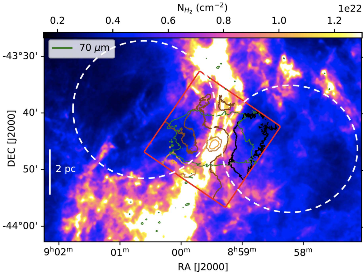
Figure 18. Herschel column density map of the region in Vela C around RCW 36 (outlined by the green 70 \mu\text{m} contour). The bipolar cavity only fills up a part of the large, low column density region around RCW 36, indicated by the dashed white circles. The black to orange contours indicate the increasing diffuse Chandra X-ray emission. This shows some hints of a correlation between the diffuse X-ray emission and the column density structure in the larger, low-density regions surrounding RCW 36, e.g., in the north and southeast of the map. The red box indicates the region covered by the Chandra data.
