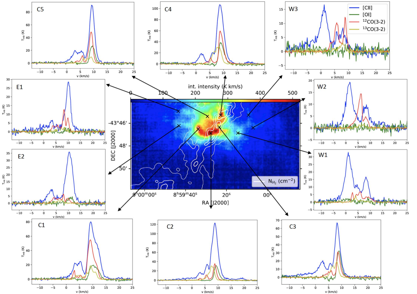
Figure 2. The middle panel shows the line-integrated intensity map of [C II] from -20 to 20 km s ^{-1} , with the white contours indicating the Herschel column density N_{\text{H}_2} at (1, 2, 4, 8) \times 10^{22} cm ^{-2} . The [C II], [O I], ^{12}\text{CO} (3–2), and ^{13}\text{CO} (3–2) spectra at the indicated positions are shown around the map. These spectra are named after their position in the map. The spectra from the central molecular ring are indicated with a “C,” the spectra to the east with an “E,” and the spectra to the west with a “W.” The spectra indicate the presence of multiple velocity components and show signatures of self-absorption toward the ring (C). In several spectra (C1–C3), high-velocity blue- and redshifted wings are detected. The spectrum “W3” at the top right highlights the color legend for the spectra. When inspecting the spectra, note that the y-scale is different in each subpanel.
