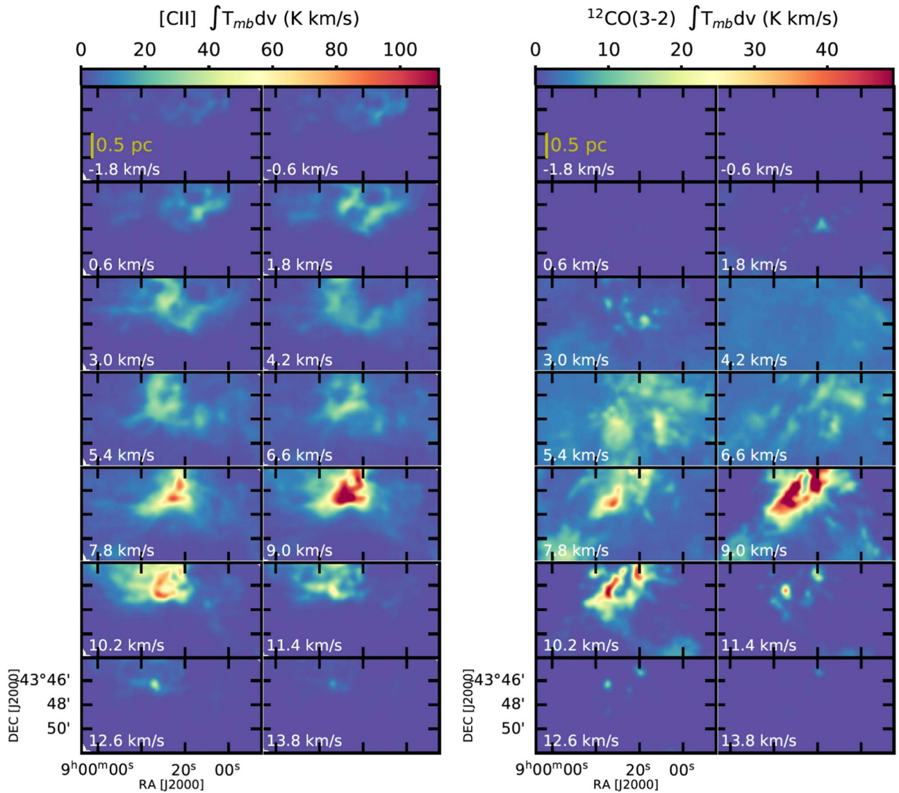
Figure 7. Left: channel maps of [C II] from -1.8 to 13.8 \text{km s}^{-1} with velocity intervals of 1.2 \text{km s}^{-1} present the velocity structure of RCW 36. Below 6 \text{km s}^{-1} , the blueshifted expanding shells are observed in the color map for [C II]. Right: same as the left panel, but for ^{12}\text{CO} (3–2) covering the same area as the [C II] map. It appears that ^{12}\text{CO} (3–2) only marginally traces the expanding shell. At higher velocities, ^{12}\text{CO} (3–2) mostly traces the kinematics of the Vela C molecular cloud.
