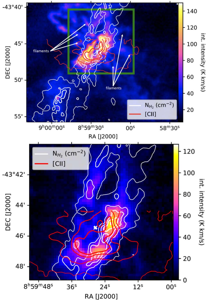
Figure 4. Top: the integrated ^{12}\text{CO} (3–2) emission map from -20 to 20 \text{ km s}^{-1} , with Herschel column density contours in white and [C II]-integrated intensity contours starting at 50 \text{ K km s}^{-1} with increments of 100 \text{ K km s}^{-1} in red to delineate their structure. Outside the molecular ring, the ^{12}\text{CO} (3–2) emission shows filamentary structures that are oriented perpendicular to the ring (indicated by the white arrows). Bottom: same as the top panel, but for ^{13}\text{CO} (3–2), in the green box indicated in the figure above, which follows the column density contours of the high column density ring closely. The [C II] emission shows a structure perpendicular to the high column density ring in the southwest at the location where there is a drop in ^{13}\text{CO} (3–2) intensity. The white crosses indicate the location of the two O-star candidates.
