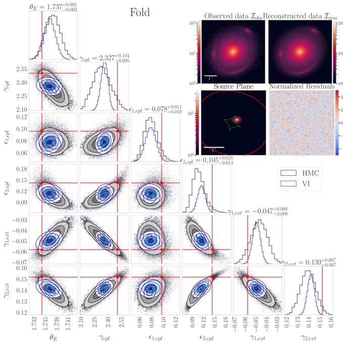
(a) Folds
