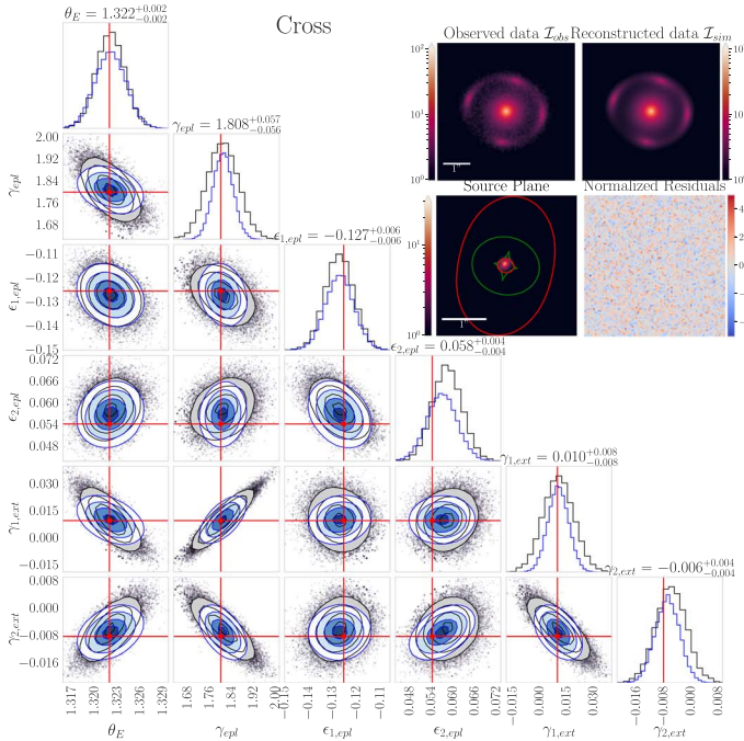
(c) Crosses
