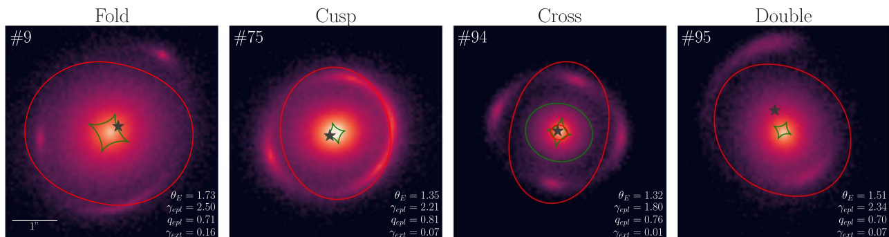
Figure A1. Four archetypal lensing systems selected from Figure 10. The numbers in the upper left corner refer to the ordering in Figure 10. All four systems have a comparable signal-to-noise ratio. The source location is marked with a star, the critical curves are in red, and the caustics are in green. Observe the presence of an inner critical curve and caustic in the cross system, due to the fact that \gamma_{\text{epl}} < 2 (e.g., O’Riordan et al. 2019).
