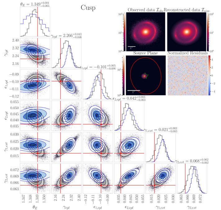
(b) Cusps
