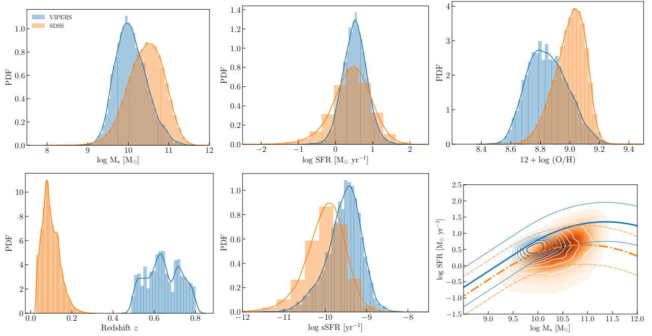
Fig. 3. Histograms and KDE of M_\star (top left), SFR (top mid), metallicity (top right), redshift (bottom left), sSFR (bottom mid), and main sequence (bottom right, with the comparison with the function described by Schreiber et al. 2015 – bold lines) for the VIPERS (blue) and SDSS (orange) samples. The thinner lines are the \pm 4 times the main sequence.
