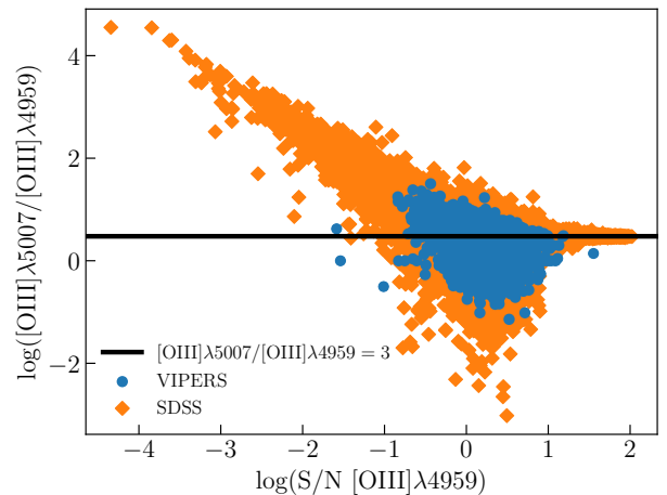
Fig. 9. Line ratio [O III] \lambda 5007 / [O \text{ III}] \lambda 4959 vs. S/N of the line [O III] \lambda 4959 for VIPERS (blue dot) and SDSS (orange diamonds) samples. The solid black line shows the intrinsic value of the line ratio.
