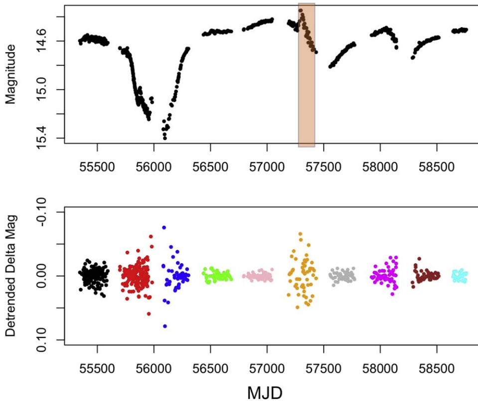
Figure 6. Top: OGLE IV optical light curve for the optical counterpart of SMC X-2. The type II outburst happened during the OGLE IV monitoring, as shown by the shaded region. Bottom: detrended light curve for each individual year.
