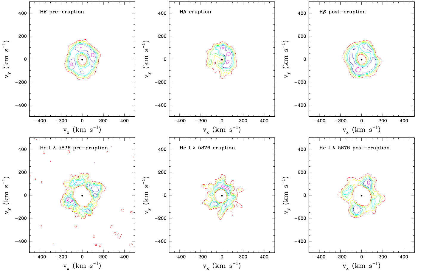
Fig. 8. Doppler maps of the H \beta (top row) and He I \lambda 5876 (bottom row) lines. From left to right the different maps correspond to the pre-eruption, eruption, and post-eruption epochs. The contours correspond to 95 (magenta), 80 (blue), 70 (cyan), 60 (green), 50 (yellow), and 40% (red) of the value of the highest peak in the map. No correction for the photospheric absorption component was applied.
