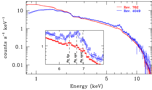
Fig. B.3. Same as Fig. B.1, but for revolution 4049 (January 2022) compared against revolution 0762.
