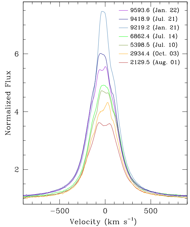
Fig. 9. H\alpha emission line profile of \gamma Cas at the different epochs of the X-ray observations discussed here. The labels indicate the date of the observation in the format HJD–2 450 000. Except for the July 2021 and January 2022 spectra (TIGRE observations), the data were taken from the BeSS database.
