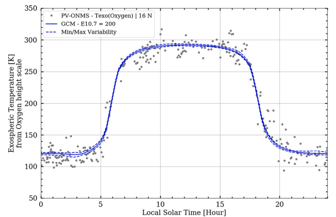
Fig. 3. Diurnal variation of the Venusian exospheric temperature derived from the oxygen height scale (grey points) and predicted by the IPSL VGCM (blue) at 16° North for E10.7 = 200 \pm 15 s.f.u. The exospheric temperature is averaged between 10^{-6} Pa and 10^{-8} Pa for the GCM. The Min/Max variability corresponds to the minimum and maximum values of the modelled temperature in the pressure range and latitude of interest. The gap between 6 and 7.5 h LT is due to the lack of data respecting the restricting conditions. (For interpretation of the references to colour in this figure legend, the reader is referred to the web version of this article.)
