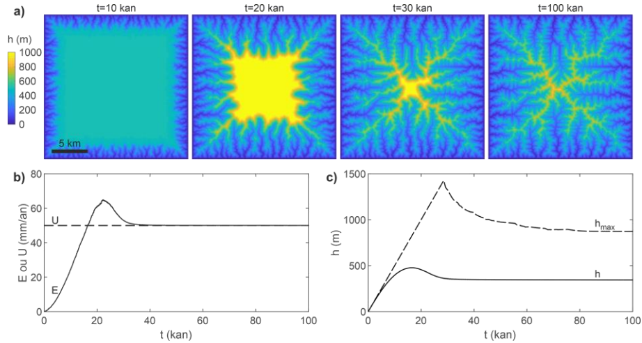
Figure 2.1. a) Maps of the temporal evolution of the topography h of a relief subject to tectonic uplift and erosion by rivers and slopes. b) Temporal evolution of the rates of uplift U and erosion E averaged over the whole model. c) Temporal evolution of the mean elevation h and maximum elevation h_{max} of the topography. Erosion rates higher than the uplift rate are obtained around 20 kyr and are explained in particular by a transient imbalance of the planar hydrological flow network during the incision of the plateau (e.g. Carretier et al., 2009).
