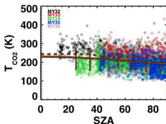
Fig. A1. Exobase temperature derived from NGIMS measurements of CO 2 scale heights made on the dayside (SZA < 90°) from 7 years of MAVEN observations. Data from MYs 32, 33, 34, 35 and 36 are shown in circles colored black, red, green, blue, and purple, respectively. The standard deviation in temperature, derived from 10° SZA bin averages, is shown in vertical brown bars. The best fit to the averages is shown as a solid brown line. The fit is compared with that of other workers (brown dotted line) (e.g., Stone et al., 2018). (For interpretation of the references to color in this figure legend, the reader is referred to the web version of this article.)
