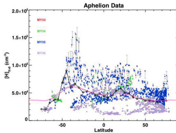
Fig. A3. Aphelion H densities as a function of latitude. These modeled densities (color coded by MY shown in the legend) have been normalized to SZA = 0^\circ . The data points were averaged over 5^\circ latitude bins (black circles and solid lines) to determine the average trend in density with latitude. The trends were smoothed to provide the fits (pink solid lines) to latitudinal variability and are not represented by a functional form. Vertical thin grey lines represent the uncertainty in the model results for each data point. (For interpretation of the references to color in this figure legend, the reader is referred to the web version of this article.)
