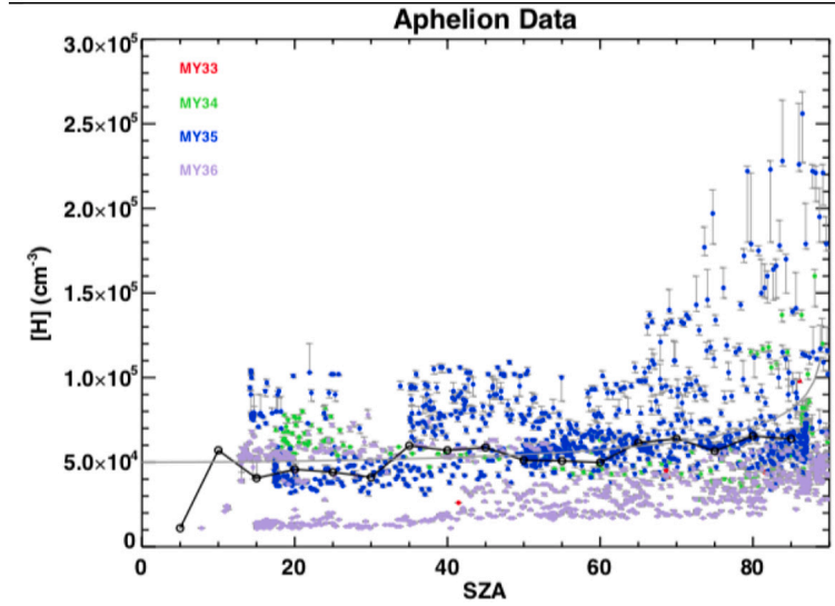
Fig. A2. Aphelion densities for H as a function of SZA. The modeled densities (color coded by Mars Year, specified in the legends) were averaged over 5^\circ SZA bins (black circles and solid lines) to determine the average trend in density with illumination conditions. The trend was used to determine a functional fit represented by Eq. A1, shown as grey solid line across the data points. Vertical thin grey lines represent the uncertainty in the model results for each data point.
