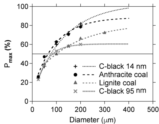
Figure 8. P_{\max} vs size of the lifted particles. C-blacks are fluffy aggregates; coals (anthracite and lignite) are solid porous particles. Horizontal line is for 50 % polarization.
