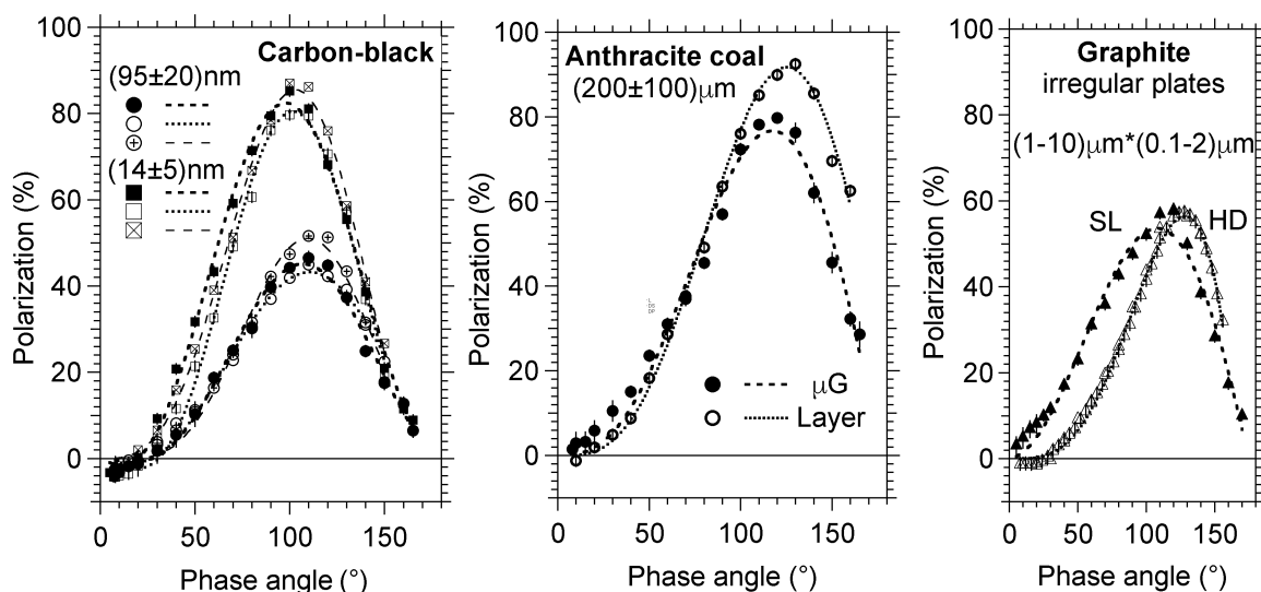
Figure 2. PPC for samples made of carbon material with different sizes for the constituent grains. Left: C-black in fluffy aggregates with constituent grains in the tens nanometres size ranges (full symbols for lifted particles, open symbols for deposited sifted particles, symbols with cross for deposited packed particles). Center: Anthracite coal in compact particles (lifted particles, layer for deposited particles). Right: graphite in agglomerates. HD=huge deposited agglomerate, LS= lifted small agglomerates). SEM images of the particles can be found in Hadamcik et al. (2002; 2006; 2007b).
