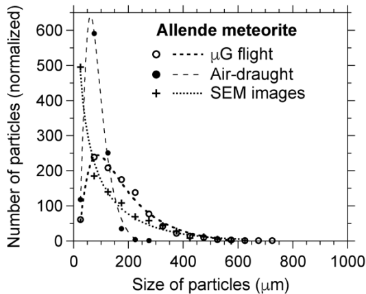
Figure 5b: Same than Fig. 5a, for Allende
