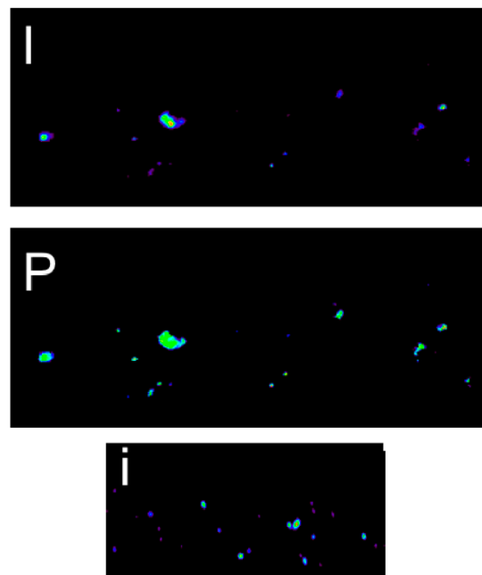
Figure 3. Orgueil meteorite particles lifted in microgravity conditions. Phase angle 90^\circ , Field of view 8 \text{ mm} \times 3.4 \text{ mm} , Intensity 'I' (up), Polarization 'P' (middle), Reference intensity 'i' map at a fixed phase angle, allowing normalization of the intensity (down). Intensity images are in arbitrary units with red for high intensities and purple for low intensities. The polarization maps are in percent, red is for 100 % polarization and purple for -50 %.
