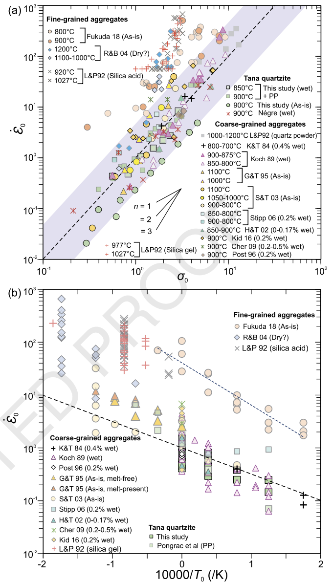
Fig. 7. Comparisons of our newly developed dislocation creep law for wet quartzite with the results of previous studies in nondimensional and semi-nondimensional spaces. To make a rational comparison with our experimental condition, we only included the results from studies that were conducted in a coaxial geometry at \geq 750^\circ\text{C} , and satisfying the Goetze criterion. a) Plot of nondimensionalized strain rate ( \dot{\epsilon}_0 ) as a function of nondimensionalized stress ( \sigma_0 ), calculated from the original mechanical data ( \sigma and \dot{\epsilon} ) as reported in the previous literature. b) Nondimensionalized strain rate ( \dot{\epsilon}_0 ) as a function of inverse temperature ( T_0^{-1} ). Acronyms used in these plots are as follows. K&T84: Kronenberg and Tullis (1984); Koch 89: Koch et al. (1989); L&P92: Luan and Paterson (1992); Post 96: Post et al. (1996); G&T 95: Gleason and Tullis (1995); H&T 02: Heilbronner and Tullis (2002); S&T03: Stipp and Tullis (?); R&B04: Rutter and Brodie (2004); Stipp 06: Stipp et al. (2006); Cher 09: Chernak et al. (2009); Kid 16: Kidder et al. (2016); Fukuda 18: Fukuda et al. (2018); Nègre: Nègre et al. (2021).
