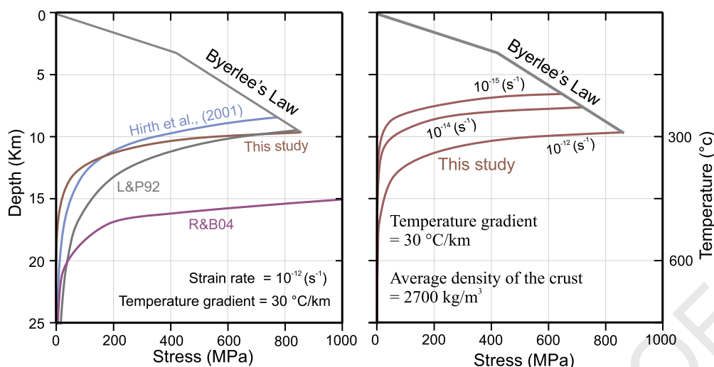
Fig. 8. A comparison between stress versus depth profile (assuming the average density of the crust as 2700 \text{ kg/m}^3 and a geotherm of 30^\circ\text{C/km} ). Our flow law predicts lower strength than popular flow laws at \dot{\epsilon} = 10^{-12} \text{ s}^{-1} . A strength variation at geologically viable strain rates is shown using our flow law. Yield stress envelopes are drawn based on the Byerlee's law (Byerlee, 1978).
