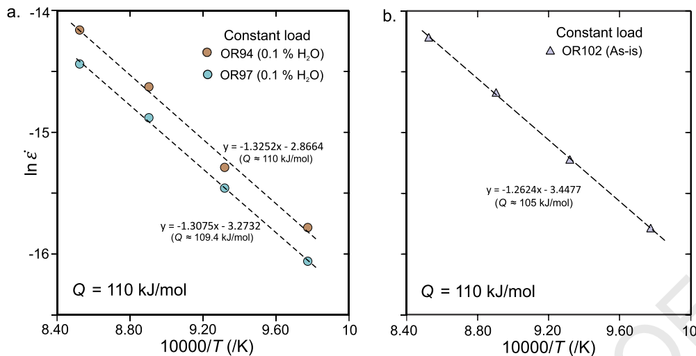
Fig. 4. Arrhenius plots of \ln(\dot{\epsilon}) against inverse of temperature ( 10000/T ) for both the H 2 O-added (a) and as-is (b) Tana quartzite. The determination of the Q -value without previous knowledge of the n -value is a great advantage of the stress-stepping-tests. Our Q -value of 110 kJ/mol is the lowest Q -value determined so far from solid-medium piston-cylinder (Table 1). However, it is in the same range of values as the studies by Kronenberg and Tullis (1984) and Paterson and Luan (1990).
