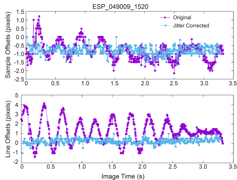
Figure 3. Plots of pixel offsets in the sample, or cross-track ( top ), and line, or along-track ( bottom ) directions, measured in the overlapping region of the RED4 and RED5 CCDs over the length of observation ESP_049009_1520. Before jitter correction (purple), pixel offsets show an amplitude of up to 4 px. After correction (light blue), offset amplitudes are reduced to \sim 0.5 px in both the sample and line directions.
