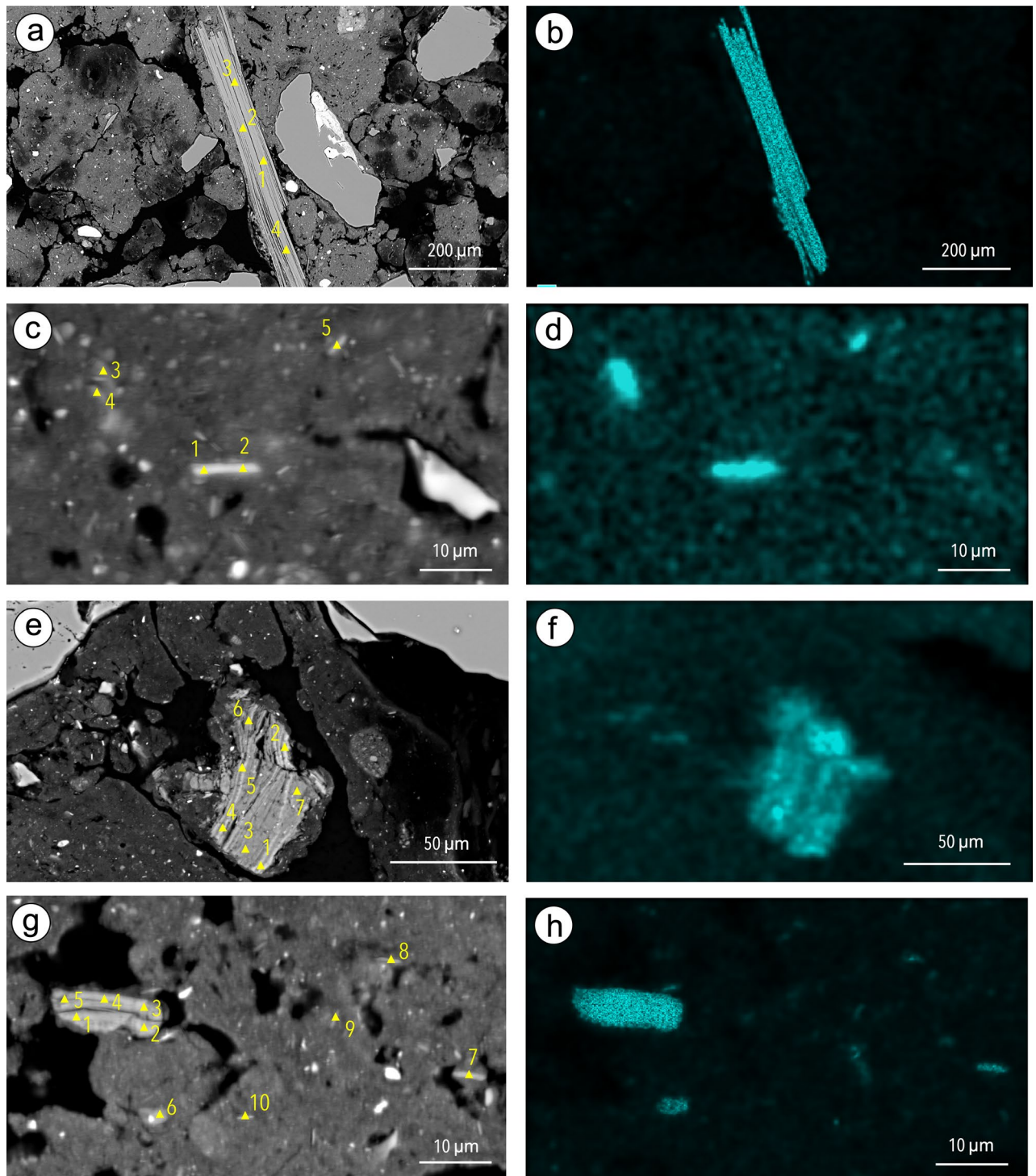
Figure 1. Elongated particles with varying sizes observed on the backscattered scanning images (BESI) of the cross sections of Ferralsols F1 (a), F2 (c), F3 (e) and F4 (g), location of the analyses (yellow triangles) performed by using energy dispersive spectrometry (EDS) (the numbers correspond to the analysis points in Supplementary Table 1), and K maps of the same areas using EDS for F1 (b), F2 (d), F3 (f) and F4 (h).
