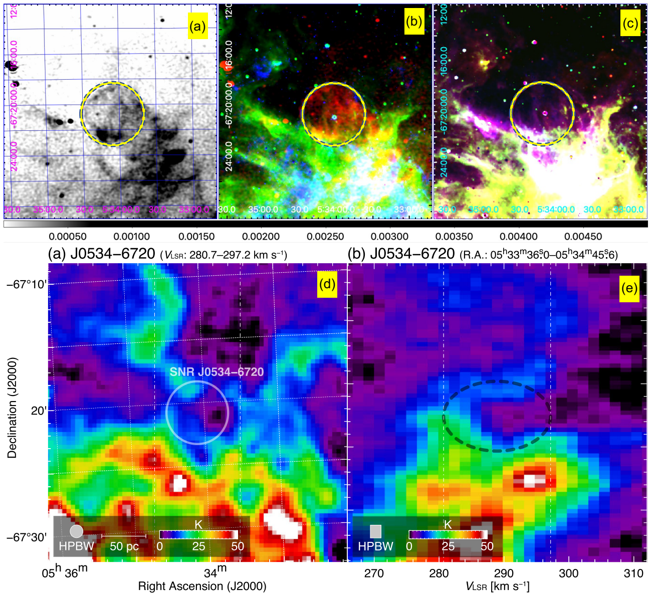
Figure A10. J0534 – 6720: same as Fig. A1. Gray scale at the bottom of Panel A is from 0 to 5 mJy beam ^{-1} . The central star visible in optical images is a Galactic foreground star HD 269767 and is not related to the source.
