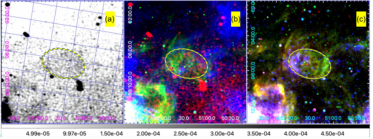
(a) J0451–6906 ( V_{\text{LSR}} : 236.2–249.4 km s ^{-1} )
