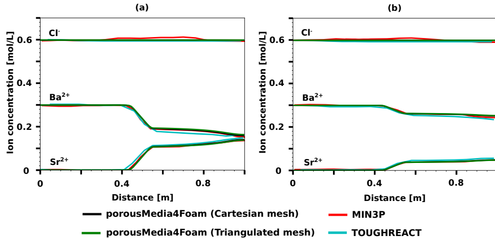
Figure 16: Case 8 – Evolution of the primary ion species –barium ( Ba^{2+} ), strontium ( Sr^{2+} ) and chloride ( Cl^- ) within the flow cell at (a) 150 hours, (b) 300 hours. The data was collected at a height of y = 0.01 m along the length of the flow cell.
