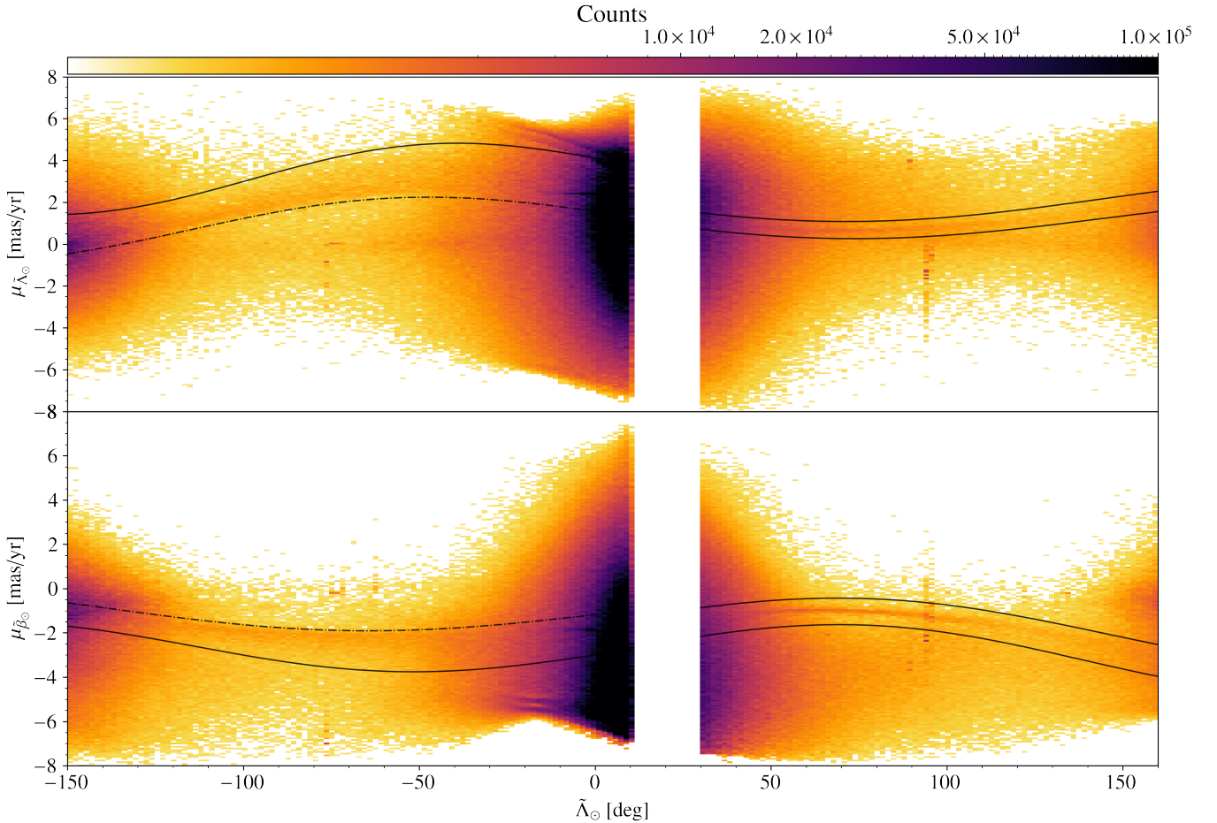
Fig. 1. Proper motion of the peaks in the Sgr celestial frame as a function of \tilde{\lambda}_{\odot} . Top : \mu_{\tilde{\lambda}_{\odot}} coordinate of the kinematic structures detected, weighted by the number of stars in each peak. Bottom : same, but in \mu_{\tilde{\beta}_{\odot}} . The footprint of the Sgr stream is clearly distinguishable in both the leading and trailing arms. In the latter, we note a sharp edge and a diffuse component above and below it ( top and bottom panels , respectively). The lines represent the upper and lower limits of our kinematic selection.
