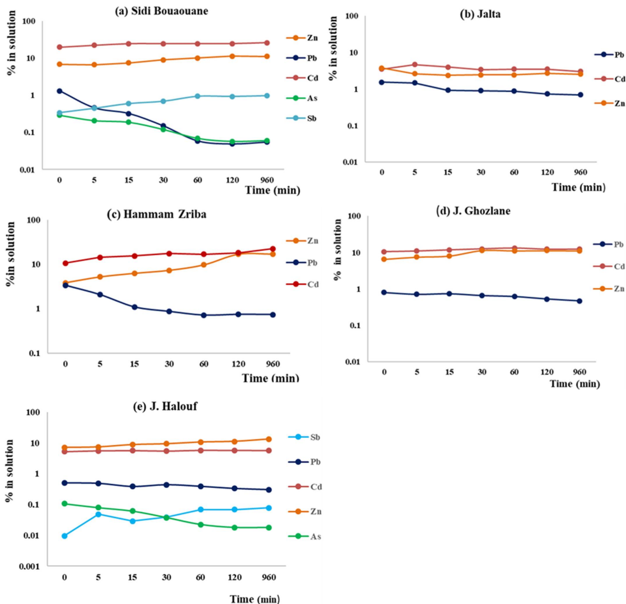
Figure 5. Evolution of the extraction rate (%) of Pb, Zn, Cd, As and Sb during the leaching test conducted on the studied soils (a): Sidi Bouaouane, (b): Jalta, (c): Hammam Zriba, (d): Ghozlane, and (e): J. halouf.
