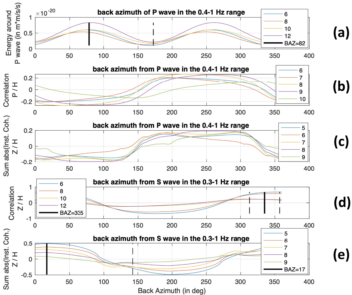
Figure A16. Back azimuth determination for event S0409d. From top to bottom: energy along the horizontal component around the P wave arrival, correlation coefficient between vertical and horizontal components around the P wave, average of instantaneous phase coherence between vertical and horizontal components around the P wave, correlation coefficient between vertical and horizontal components around the S wave, average of instantaneous phase coherence between vertical and horizontal components around the S wave. For each panel, all possible back azimuths are examined and various window length (in s) are tested (different colors). Best estimates of back azimuth are identified by vertical black lines. The error on the back azimuth estimate is computed by averaging this standard deviation and the average width of the correlation function at 80% of its peak value.
