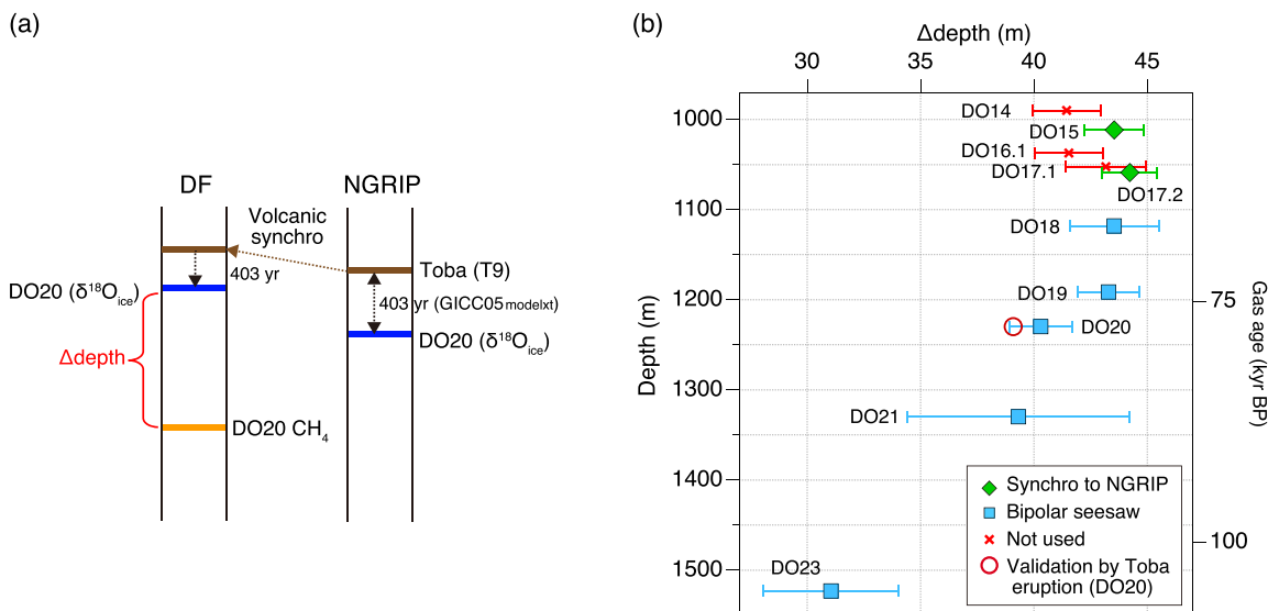
Fig. B1. (a) Schematic of \Delta depth estimation for DO 20 based on Toba volcanic matching, and (b) enlarged view of Fig. 5.
