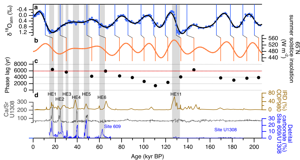
Fig. 11. Phasing between \delta^{18}\text{O}_{\text{atm}} and 65°N summer solstice insolation. (a) \delta^{18}\text{O}_{\text{atm}} of the DF core (Kawamura et al., 2007) on the DF2021 gas age scale with its filtered curve. (b) 65°N summer solstice insolation. Vertical lines in (a) and (b) indicate midpoints between maxima and minima. (c) Lag of \delta^{18}\text{O}_{\text{atm}} behind 65°N summer solstice insolation for the midpoints. Horizontal red line indicates the constant lag of 5.9 kyr typically used for \delta^{18}\text{O}_{\text{atm}} -orbital age markers (Bazin et al., 2013). (d) IRD percentage at site ODP980 (brown: McManus et al., 1999), Ca/Sr ratio, an indicator of detrital carbonate, at site U1308 (black: Hodel et al., 2008) and detrital carbonate percentage at site 609/U1308 (blue: Obrochta et al., 2012, 2014). (For interpretation of the references to colour in this figure legend, the reader is referred to the Web version of this article.)
