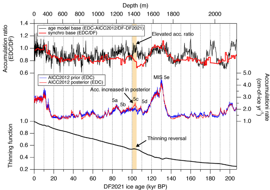
Fig. A5. Anomalous accumulation rate and thinning in the EDC core around 100 kyr BP from posteriors of AICC2012, as possible indicators for errors in \delta^{18}O_{atm} gas age markers. (a) Ratio of posterior of accumulation rate for the EDC core (from AICC2012, Veres et al., 2013; Bazin et al., 2013) to that for the DF core (from DF2021), and the ratio based on detailed age synchronization between the cores (Parrenin et al., 2016). (b) Accumulation of the prior (blue) and posterior (red) of the EDC core in the AICC2012 chronology (Parrenin et al., 2007b; Veres et al., 2013; Bazin et al., 2013). (c) Thinning function of the EDC core in the AICC2012 chronology (Veres et al., 2013; Bazin et al., 2013).
