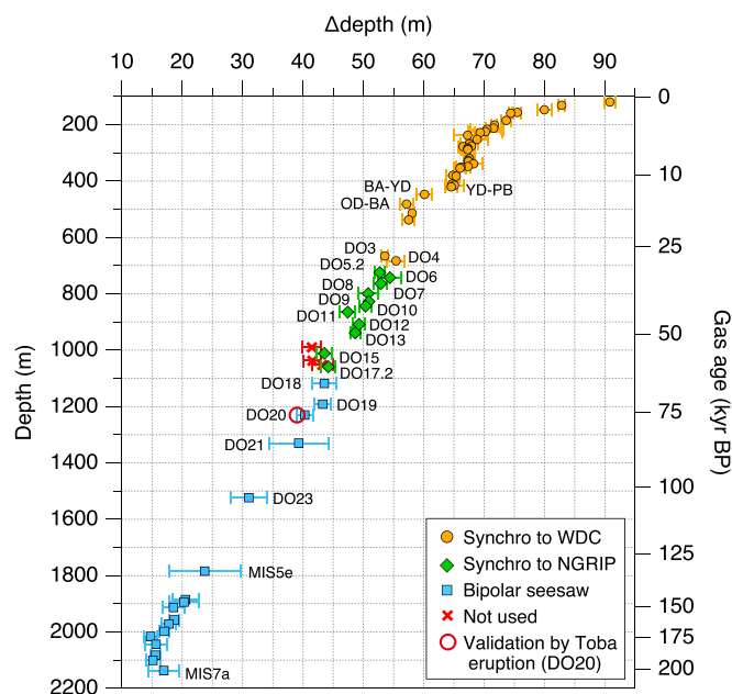
Fig. 5. Empirical Δdepth for the DF core based on the ice and gas synchronizations to the WDC and NGRIP core, or synchronicity between AIM and CH 4 transitions under the bipolar seesaw assumption. Δdepth for DO 14, 16.1 and 17.1 are not used for the age construction (see text). Also shown is a validation point for DO 20 by the Toba bipolar volcanic matching (Svensson et al., 2013) (see Appendix B for details).
