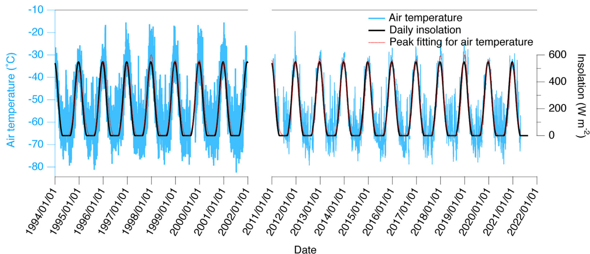
Fig. A2. Comparison between daily mean insolation (calculated with the AnalySeries software using the Laskar et al., 2004 solution) and air temperature observed by an automatic weather station (Takahashi et al., 2004; Morino et al., 2021) at Dome Fuji, Antarctica. A general peak fitting algorithm (“Multipeak Fitting 2” package of Igor Pro®) was used for identifying the timing of summer temperature peaks (see text).
