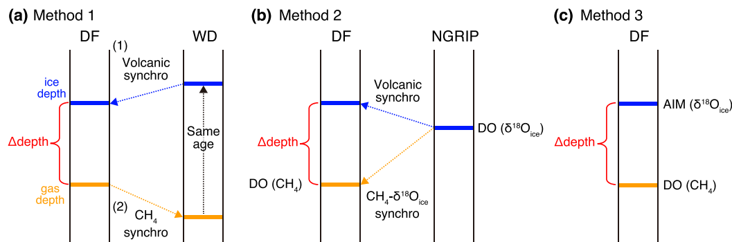
Fig. 4. Schematic of three methods for estimating Δdepth (see text for detailed explanation). DF: Dome Fuji, WD: WAIS Divide.
