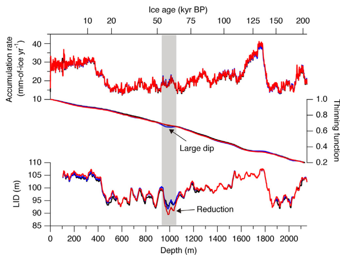
Fig. A3. Comparison between the A , \tau , and LID with (red and blue) and without (black) \Delta depth constraints for D014, 16.1 and 17.1. If relatively large uncertainty of \tau is assigned (before Step 2, increased linearly from the ice-sheet surface (0%) to the bottom (100%)), a large dip is produced in \tau (blue). On the other hand, if the smaller uncertainty of \tau (the result from Step 2) is assigned, shallowing of LID is produced (red).
