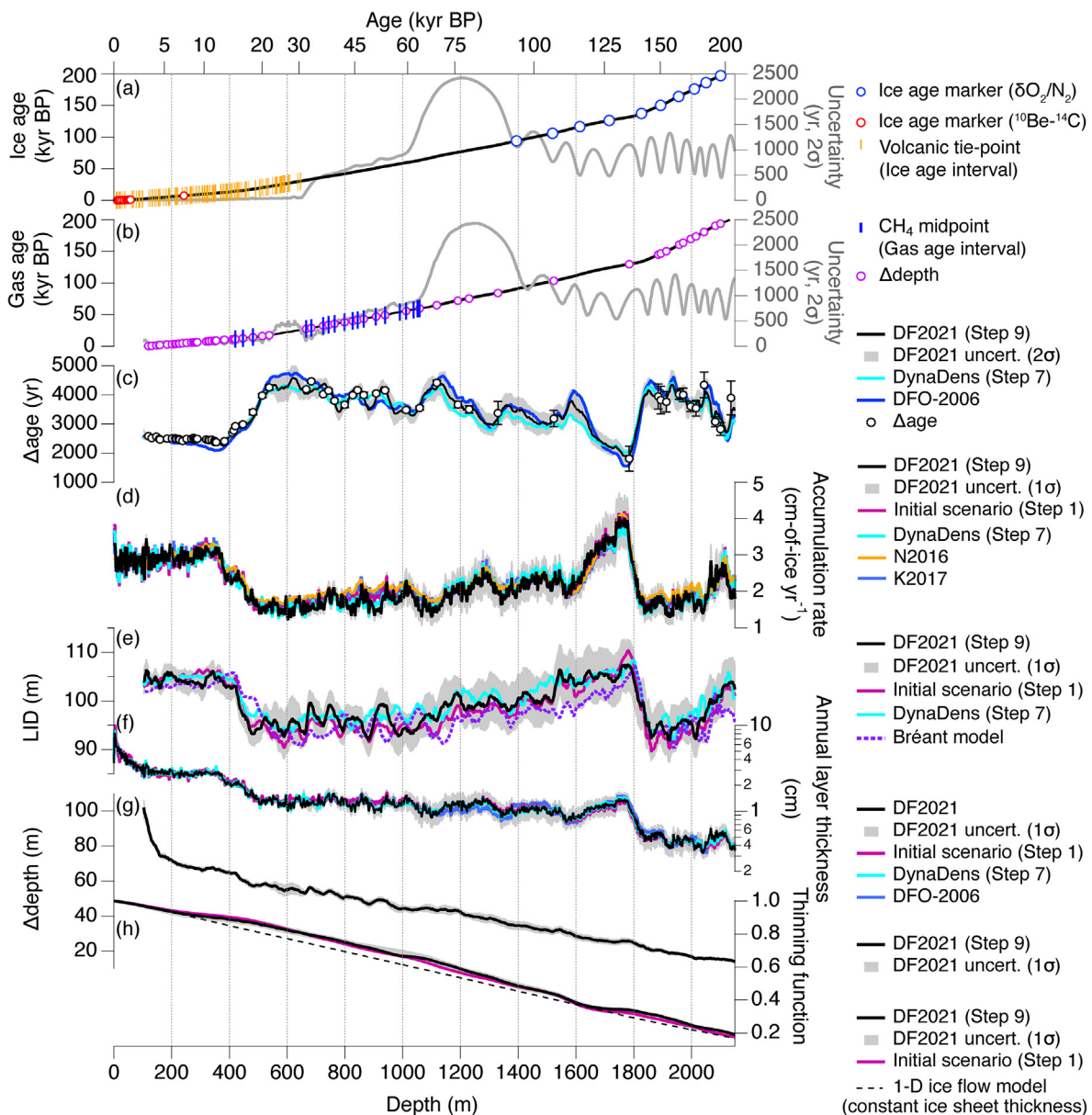
Fig. 6. The DF2021 chronology and associated glaciological parameters. (a) Ice age scale with 2σ uncertainty, and ice age constraints. (b) Gas age scale with 2σ uncertainty, and gas age and Δdepth constraints. (c) Δage with 2σ uncertainty, intermediate Δage from the firn model, and previous Δage in DFO-2006 (Kawamura et al., 2007). (d) Accumulation rate with 1σ uncertainty, initial scenario, intermediate scenarios from firn models, and previous studies (Nakano et al., 2016; Dome Fuji Ice Core Project Members, 2017). (e) Same as (d) but for annual layer thickness. (g) Δdepth with 1σ uncertainty. (h) Thinning function with 1σ uncertainty, initial scenario, and model result with constant ice thickness.
