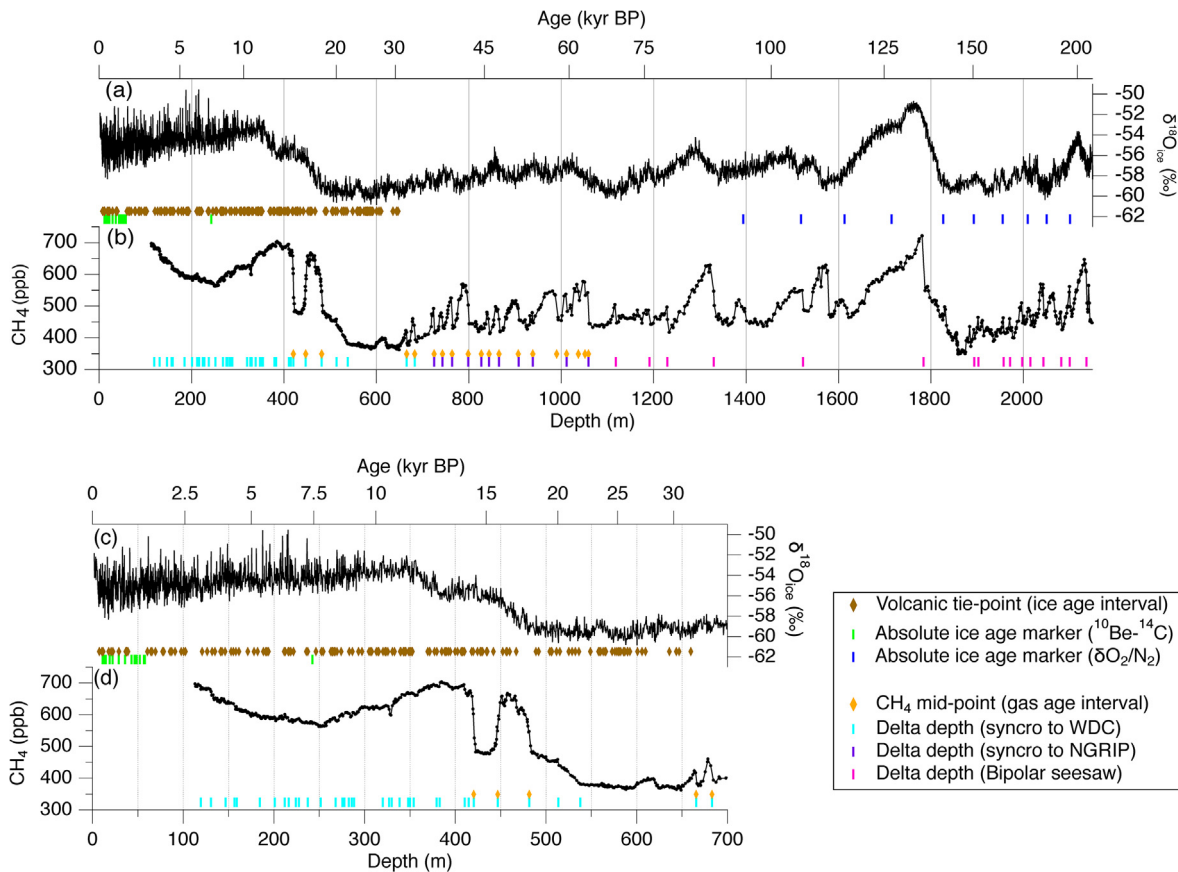
Fig. 2. Age constraints for ice and gas in the DF core. (a) Ice age constraints with \delta^{18}O_{ice} as reference (Dome Fuji Ice Core Project Members, 2017). Different markers indicate the volcanic horizons for intervals between neighboring ice age markers (ice age intervals), ^{10}Be absolute age markers, and \delta O_2/N_2 age markers. (b) Gas age constraints with CH_4 record as reference. Different markers indicate the CH_4 transitions (for DO events and minor wiggles) for deducing intervals between neighboring gas age markers (gas age intervals) or \Delta depth through the synchronization to WDC or NGRIP core (for 0–65 kyr BP), or through bipolar-seesaw assumption (>65 kyr BP). (c) and (d) Enlarged views of (a) and (b), respectively.
