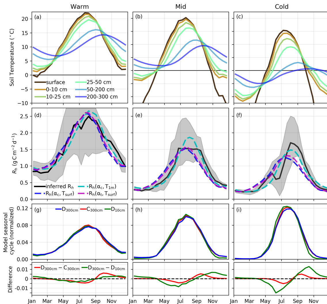
Figure 5. Impact of temporal and vertical variations in carbon pools on R_h . (a–c) MERRA-2 Land soil temperature over five intervals for the (a) Warm, (b) Mid, and (c) Cold regions. (d–e) Mean and range in inferred 14 d R_h with fits for single-layer R_h models that employ (navy dash) T_{\text{surf}} dependence and no seasonal variations in the carbon pool, (cyan dash) T_{1m} dependence and no seasonal variations in the carbon pool, and (magenta dash) T_{\text{surf}} dependence and seasonal variations in the carbon pool. (g–i, top) Normalized seasonal cycle of R_h simulated by the soil decomposition model (Sect. 2.6). The different lines show different model simulations: D_{300\text{cm}} employs a dynamic carbon pool over 0–300 cm depth, C_{300\text{cm}} employs a constant carbon pool over 0–300 cm depth, and D_{10\text{cm}} employs a dynamic carbon pool over 0–10 cm depth. (g–i, bottom) Differences in simulated R_h between experiments.
