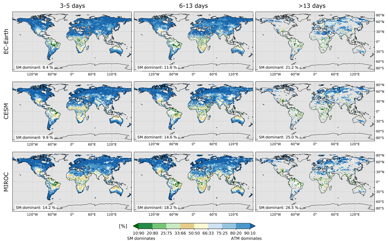
Figure 8. Contribution of atmospheric circulation (ATM) vs. soil moisture (SM) to warm spells during the local summer season when daily mean temperature anomalies exceed 1.5 SD (standard deviation) from the ERA-Interim 1981–2010 climatology. The local summer season is defined as the hottest consecutive 3 months (from ERA-Interim) for each grid point. The two approaches to compute the SM vs. ATM contribution are merged, giving equal weight to both. Events are categorized into spells lasting 3–5 d, 6–13 d, and 14 d or longer. Ocean grid points, Antarctica, Greenland, and Iceland are masked out in grey using the Greenland–Iceland (GIC) region from the AR6 reference regions for the latter two. Grid points for which no events were identified are also masked out in grey. Grid points for which the contributions could not be determined (see text) are masked out in white. In the lower left corner the grid points for which the SM contribution dominates over the ATM contribution ( > 50\% ) are given as an area-weighted percentage with respect to all valid grid points.
