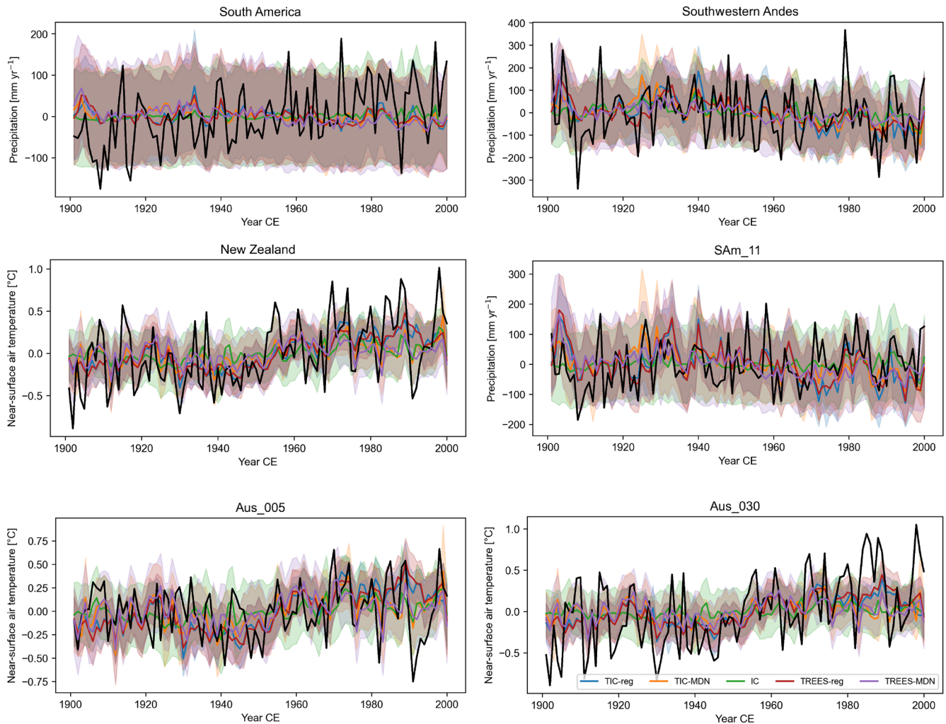
Figure 6. Reconstructed (in color) and GMF (in black) temperature (in °C; relative to 1901–2000 CE) or precipitation anomalies (in mm yr -1 ; relative to 1901–2000 CE) over 1901–2000 CE for different DA experiments (Table 1, with ice core proxies only, with tree-ring proxies only or with both) in different regions (Sect. 3) and proxy sites (Fig. 1). Aus refers to a site in New Zealand and SAM in South America. The uncertainty (i.e., the ensemble spread; Sect. 2.1) associated with each reconstruction is represented by the shaded areas.
