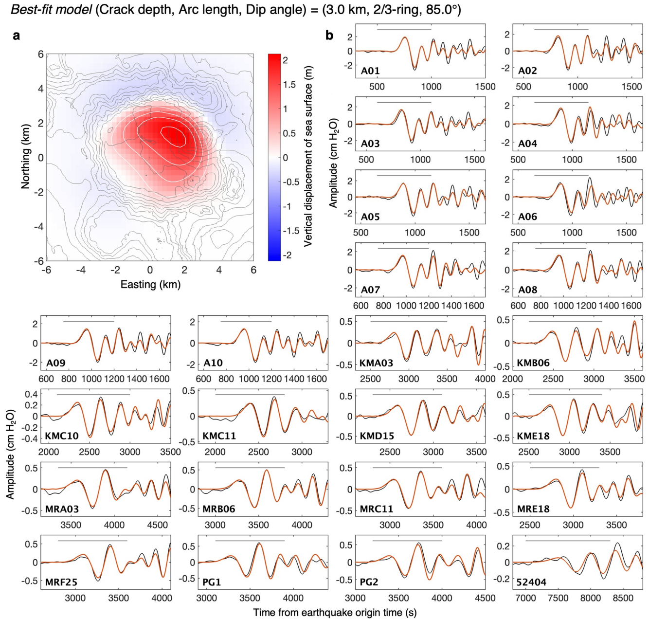
Figure 6. Tsunami waveforms from the best-fit source model (Figure 4a). (a) Vertical displacement of sea surface caused by the model. Red and blue colors represent uplift and subsidence, respectively, with white contour lines plotted every 0.5 m. Note that the color scale in this figure is different from that in Figure 2a. (b) Comparison of the observed (black) and synthetic (red) tsunami waveforms from the model at the ocean bottom pressure gauges. The gray line represents the time interval used for the inversion.
