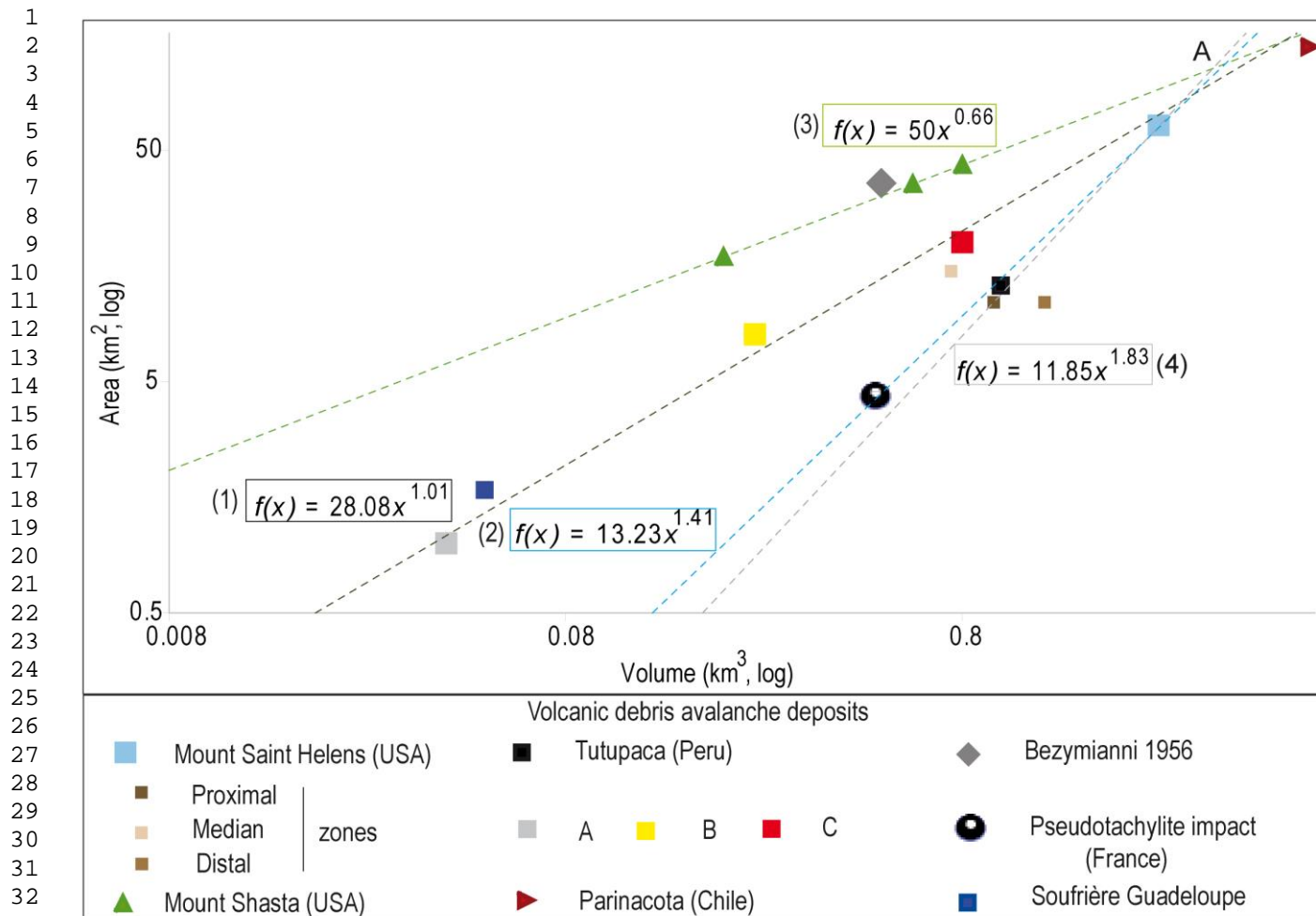
35 36 Fig. 2. Area ( \text{km}^2 ) vs. volume ( \text{km}^3 ) of volcanic debris avalanche deposits on double log graph: Mount 37 Shasta and Mount Saint Helens in the USA (Glicken, 1986; Siebert et al., 1987); Bezymianni in Kamchatka 38 (Siebert et al., 1987); Parinacota in Chile (Clavero et al., 2002; Legros, 2002); Tutupaca in Peru (Samaniego 39 et al., 2015; Valderrama et al., 2016); Soufrière in Guadeloupe (Boudon et al., 1984) and Mont Dore in 40 French Massif Central (Bernard and van Wyk de Vries, 2017). A. The proximal zone; B. The ridged unit; C. 41 The distal zone. 42 43 44 45 46 47
