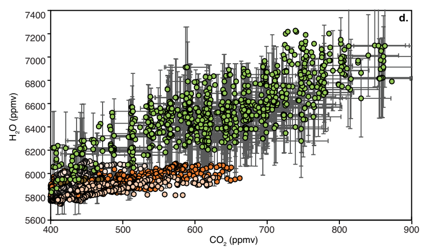
CO 2 measurements. c-d: Plot of (c) CO 2 vs. SO 2 and (d) H 2 O vs CO 2 for vent gases on the 25th March and 5th April. The measurements were carried out using a Multi-GAS device at 50-150 m from the vent source. Error bars are included on all plots and include external 2σ error.
