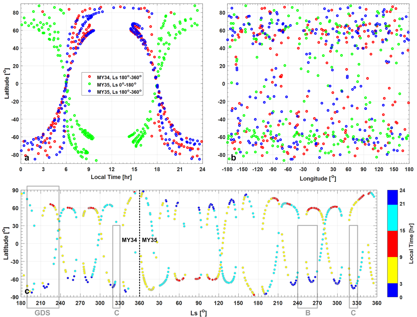
Figure 2. Geographical distributions of the tangent points for the Atmospheric Chemistry Suite MIR solar occultations at the grating position #4 covering the 2.7 \mu\text{m} band. The coordinates are latitude versus (a) local time, (b) longitude, and (c) solar longitude, L_s . The data in panels (a and b) are combined in annual periods: Second half of MY 34 (red), first half of MY 35 (green), and second half of MY 35 (blue). The data at panel (c) are color-coded by intervals of local time in hours (hr): 3–9 (yellow), 9–15 (red), 15–21 (purple), and 21–3 hr (blue). Each circle corresponds to one occultation with related coordinates of the tangential point. Gray frames in panel (c) outline periods of the global dust storm and the C storm in MY 34 and the B and C storms in MY 35.
