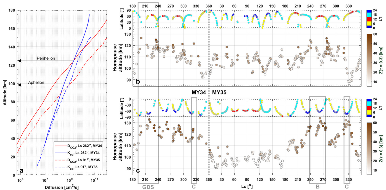
Figure 6. Revealing of the homopause altitude from the Atmospheric Chemistry Suite MIR occultations for 1.5 MYs. (a) Vertical profiles of the molecular ( D_{\text{CO}_2} , in red) and eddy ( K_{\text{ed}} , in blue) diffusion coefficients retrieved from the observations at perihelion MY 34 (solid lines) and aphelion MY 35 (dashed lines). Black arrows point to the definition of the homopause heights. (b) Distribution of the homopause altitude versus solar longitude ( L_s ) in the Northern Hemisphere; the color code corresponds to an altitude ( Z ) where the aerosol slant opacity ( \tau ) equals 0.3. The data are supplemented by the latitudinal coverage taken from Figure 2c. (c) Panel (b) shows the same for the Southern Hemisphere. Gray frames outline periods of the global dust storm and the C storm in MY 34 and the B and C storms in MY 35.
