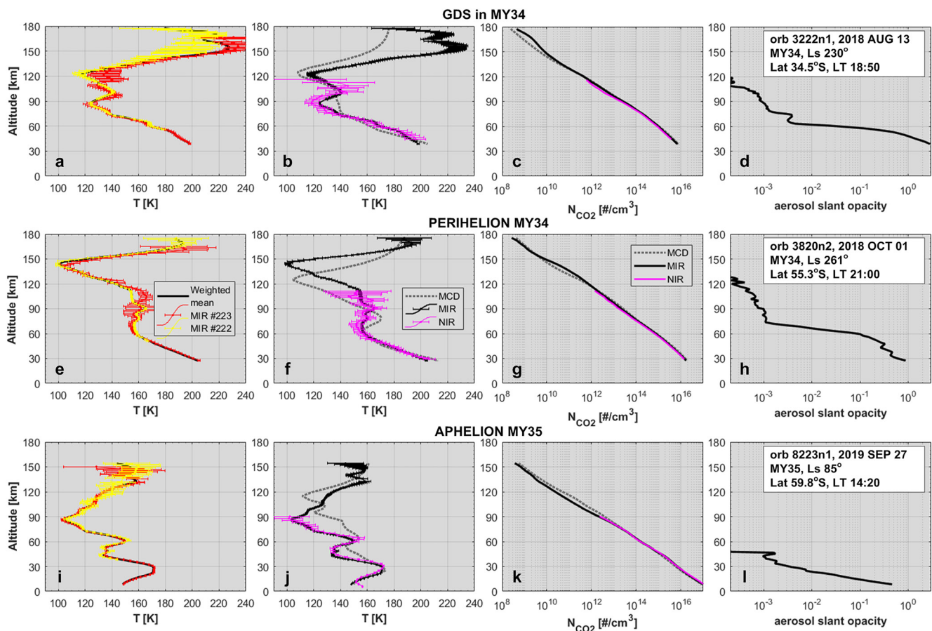
Figure 4. (a, b, e, f, i, and j) Individual vertical profiles of temperature, (c, g, and k) CO 2 number density, and (d, h, and l) aerosol slant opacity retrieved from Atmospheric Chemistry Suite (ACS) MIR occultations in the Southern Hemisphere at different periods: (a–d) global dust storm in MY 34 ( L_s = 230^\circ ), (e–h) near perihelion in MY 34, and (i–l) near aphelion in MY 35. Panels (a, e, and i) comparison between ACS MIR orders #222 (yellow) and #223 (red) with their weighted mean temperatures (black). Panels (b, f, and j): comparison of the ACS MIR temperature profiles (black) with the ACS NIR ones (magenta; Fedorova et al., 2022) and with the MCD5.3 climatology predictions (gray). Panels (c, g, and k) analogous comparison for CO 2 number density.
