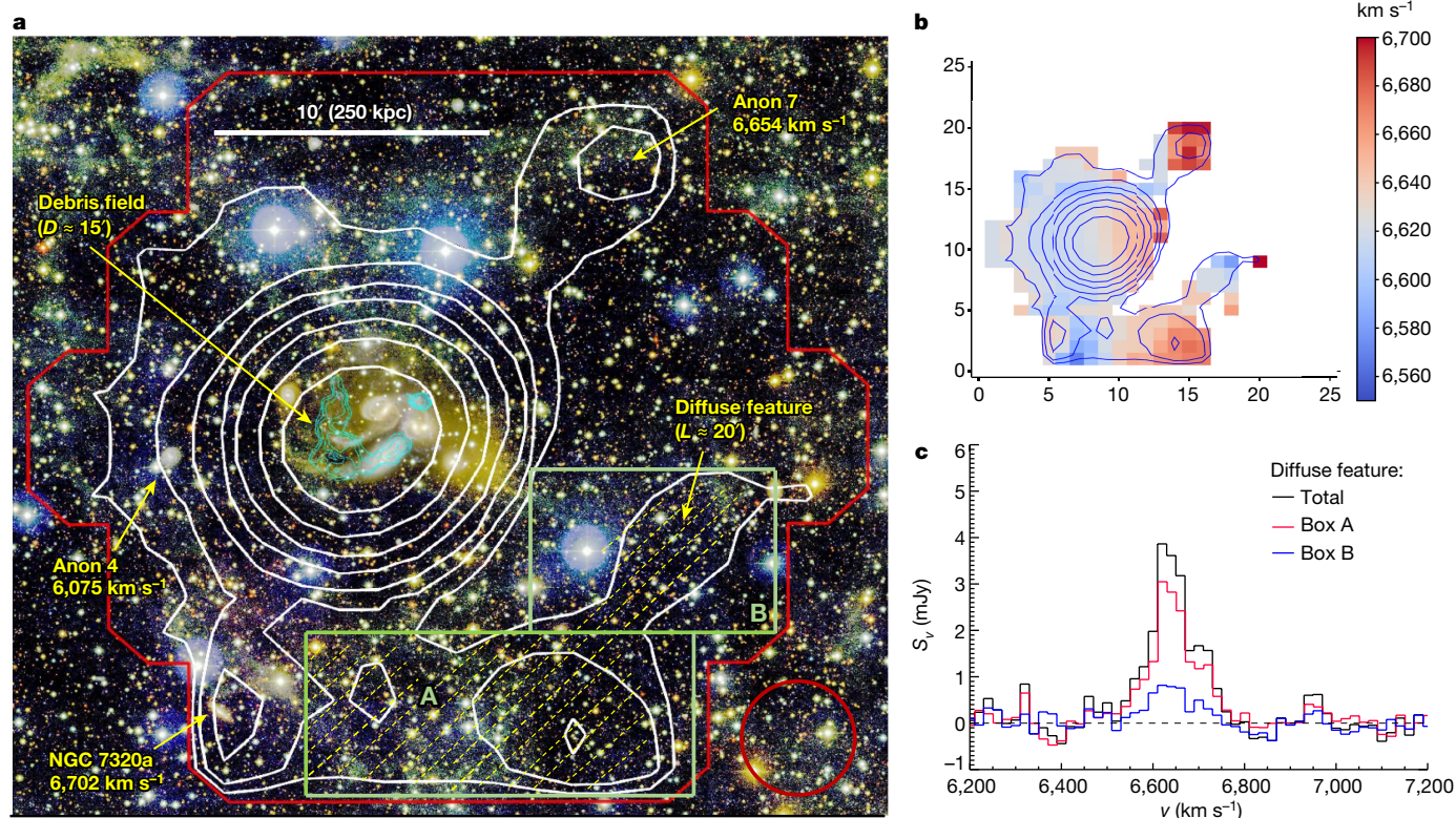
Fig. 3 | The H I emission in the velocity range of 6,550–6,750 km s -1 . a , Contour map of the integrated H I emission in the velocity range of 6,550–6,750 km s -1 overlaid on the composite colour image (u, g, r) of the deep CFHT MegaCam observation. The red circle at the bottom right illustrates the angular resolution (half-power beam size = 4.0') of the FAST map after smoothing. The contours start from N_{\text{HI}} = 7.4 \times 10^{17} \text{ cm}^{-2} (at 5.5\sigma level) with an increment of a factor of 2. The red lines delineate the boundary of the FAST observations. The cyan contours in the centre are adopted from the VLA observations for the 6,600 km s -1 component of SQ 8 , with angular resolution of 19.4'' \times 18.6'' . They have the base level at N_{\text{HI}} = 5.8 \times 10^{19} \text{ cm}^{-2} and the increment of a factor of 2. The area occupied by the newly discovered diffuse feature is
