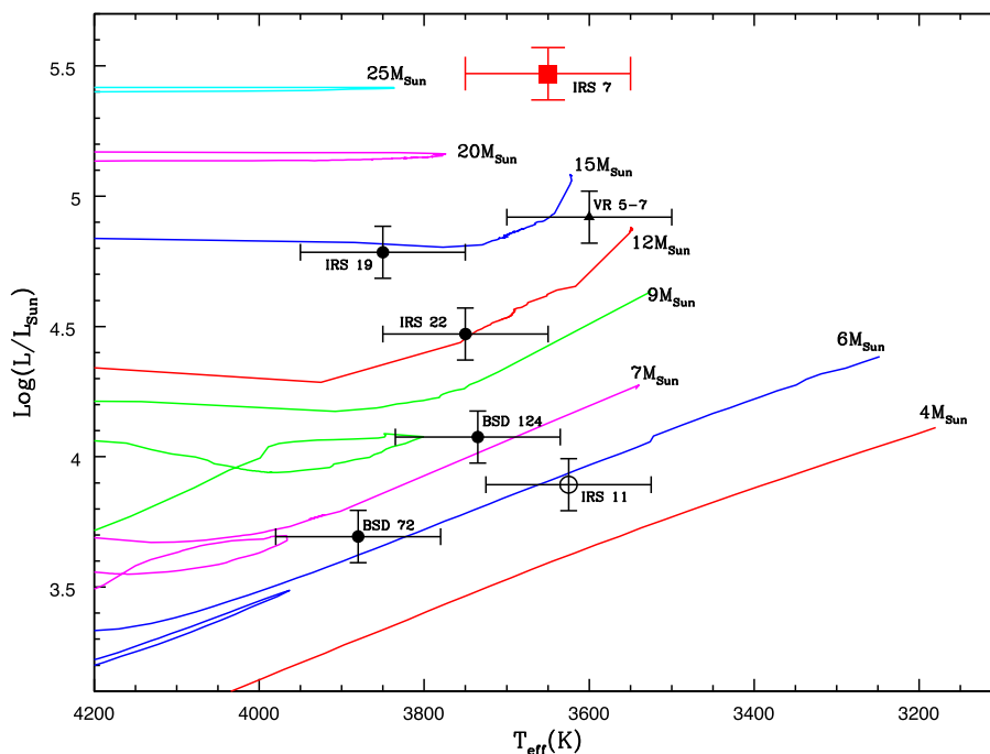
Figure 4. Luminosity [as \text{Log}(L/L_{\odot}) ] versus T_{\text{eff}} for the Galactic Centre stars discussed here. The filled and open circles are all members of the NSC, as is IRS 7, while VR 5-7 (filled triangle) is a member of the Quintuplet Cluster. The 7-, 9-, 12-, 15-, 20- and 25- M_{\odot} stellar models are rotating models from Ekström et al. (2012), while the 4- and 6- M_{\odot} stellar models are from Lagarde et al. (2012). This figure presents both the observed stars and stellar models in an evolutionary context within a type of HR Diagram.
