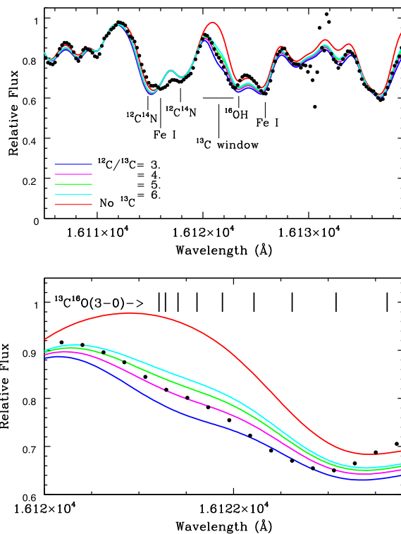
Figure 2. The top and bottom panels illustrate synthetic (continuous coloured lines) and IRS 7 (black filled circles) spectra centred on the ^{13}\text{C}^{16}\text{O}(3-0) bandhead, with five synthetic spectra having different carbon-13 abundances (one with no ^{13}\text{C} and four with ^{12}\text{C}/^{13}\text{C} = 3, 4, 5, and 6 ). The top panel provides a 35 Å-wide window of the spectral region around the ^{13}\text{C}^{16}\text{O} bandhead in order to provide a view of the overall absorption in IRS 7 and how this compares to the absorption from ^{13}\text{C}^{16}\text{O} lines. The glitch in the IRS 7 spectrum at \lambda 16130 Å is caused by poor telluric subtraction. The bottom panel is a close-up of the bandhead and illustrates the IRS 7 pixels that are most sensitive to the ^{12}\text{C}/^{13}\text{C} ratio; the isotopic ratio was set by this spectral interval from \sim \lambda 6120 – 6123 Å, resulting in \langle ^{12}\text{C}/^{13}\text{C} \rangle = 5.3 \pm 0.8 . The line positions of the individual ^{13}\text{C}^{16}\text{O} lines are illustrated by the vertical lines at the top of the bottom panel. The red end of the ^{13}\text{C}^{16}\text{O} bandhead is blended with a strong OH line plus an Fe I line (with an uncertain gf-value) further to the red.
