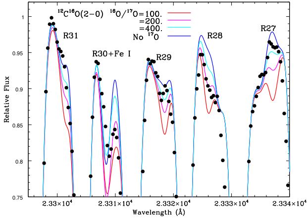
Figure 3. A 45-Å-wide spectral window illustrating the ^{12}\text{C}^{17}\text{O} lines used to estimate the ^{16}\text{O}/^{17}\text{O} ratio for IRS 7. Synthetic spectra, with different values of ^{16}\text{O}/^{17}\text{O} as noted in the plot key, are shown as solid coloured curves, with the observed IRS 7 spectrum plotted as solid black circles. This region contains the ^{12}\text{C}^{17}\text{O}(2-0) R27, R28, R29, R30, and R31 lines, with all of them blended to some degree with a number of strong ^{12}\text{C}^{16}\text{O}(2-0) and (3-1) lines running through this region. Due to this significant blending, the derived ^{17}\text{O} abundance (presented as the ^{16}\text{O}/^{17}\text{O} ratio) in IRS 7 is uncertain, although the ^{17}\text{O} isotopic lines are detected clearly.
