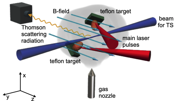
Fig. 1. Setup of the experiment, conducted at LULI2000 by having two high-power lasers (1 ns, 100 J at 1\omega , 1.6 \times 10^{13} \text{ W cm}^{-2} on target) irradiate two solid (Teflon, \text{C}_2\text{F}_4 ) targets to investigate the interpenetration of two magnetized shocks. An auxiliary beam of 15 J was used to perform Thomson scattering (TS) and an additional low-energy beam (not shown) probed the plasma along a line tilted 9^\circ upwards with respect to the z -axis in order to measure the integrated plasma electron density.
