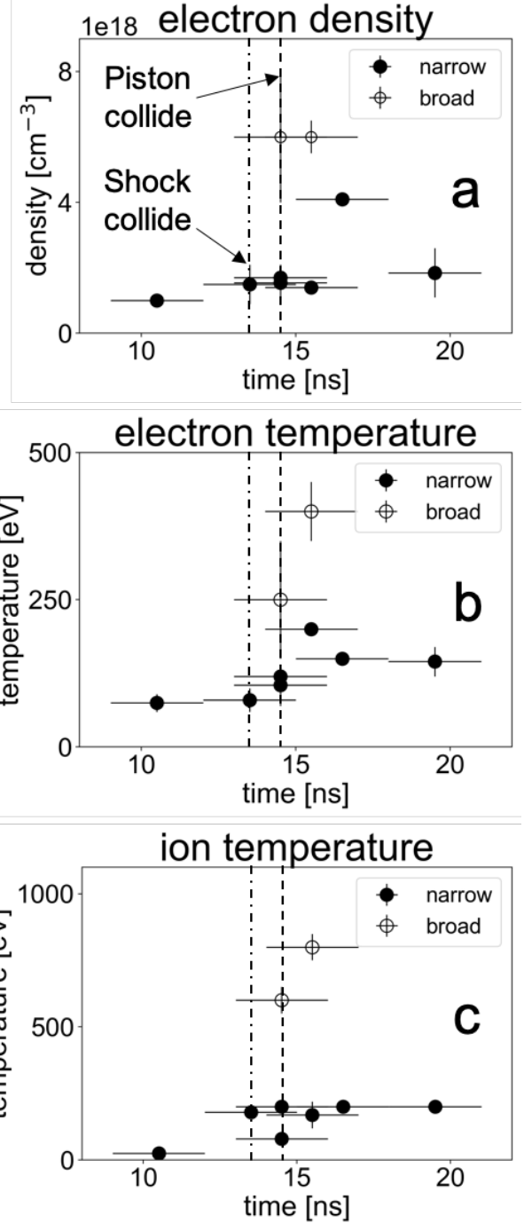
Fig. 6. TS measurements of the temporal evolution of electron density (a), electron temperature (b), and ion temperature (c). The narrow and broad configurations are respectively related to the ambient and piston plasmas (for more details, see Fig. 5 caption).
