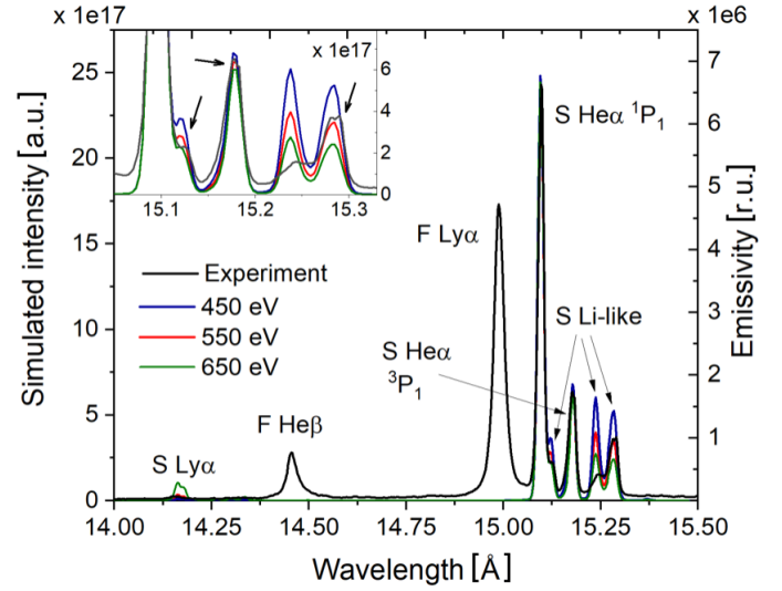
Fig. 3. Experimental x-ray spectrum (black line) measured by the FSSR spectrometer as emitted from a \text{C}_2\text{F}_4 target. What is recorded is the spectrum of sulfur impurities in the third order of reflection. Overlaid are simulations performed using the PrismSPECT code (red, olive, and blue curves) for the target surface region, using the group of satellites sensitive to the plasma parameters. For all temperatures shown in the figure, the electron density was N_e = 7 \times 10^{20} \text{ cm}^{-3} . All curves are normalized to the \text{S He}\alpha line. The best fitting corresponds to the red curve. The inset shown in the top left corner demonstrates the detailed fitting of the satellites of the experimental spectrum. The arrows point to the lines with the best fit.
