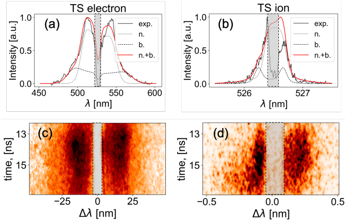
Fig. 5. Thomson scattering measurements of the plasma density and temperatures in the region of shock collision. Spectra of Thomson scattering off electron plasma waves (a, c) and ion acoustic waves (b, d). Then, (a) and (b) show the spectra profiles, corresponding to 15 ns, while (c) and (d) show the temporal evolution of the scattering spectra over a time period from 13 ns to 16 ns for the electron plasma and ion acoustic waves, correspondingly. Black solid lines (in a and b) are for experimental data profiles, while red solid lines are for theoretical spectra, composed of a superposition of narrow (black dotted lines) component relative to the ambient medium, having density 1.5 \times 10^{18} \text{ cm}^{-3} , electron temperature 100 eV, ion temperature 200 eV, and broad (black dashed lines) component relative to the piston plasma, having density 6 \times 10^{18} \text{ cm}^{-3} , electron temperature 300 eV, ion temperature 100 eV. The ratio between the magnitudes of the narrow and broad components is 3.5. We note that the deep central dip in the experimental spectra (a, b) and the white vertical region in the streak-camera images (c, d) is related to a filter (a black aluminum stripe) which is positioned right before the entrance of the two streak cameras (recording respectively the light scattered off the electron and ion waves). This filter is used to block the very intense and unshifted laser wavelength (the Rayleigh-scattered light), which otherwise would saturate the cameras. Thus, no signal is recorded in this zone, which is materialized by the gray dashed box.
