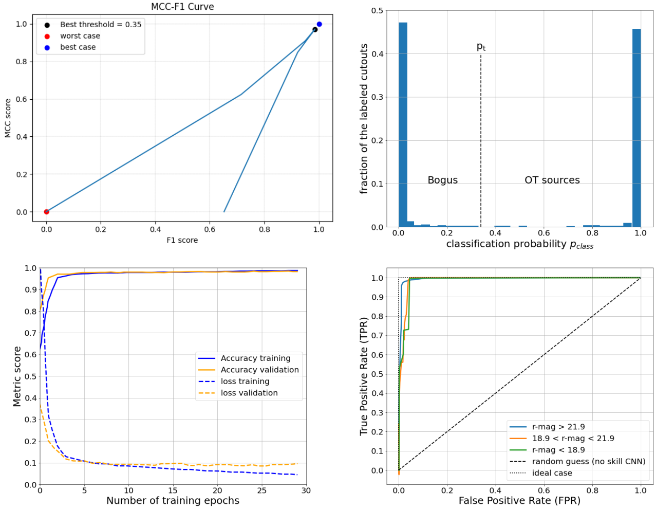
Fig. 10. Different visualisation of the metrics used to evaluate the performance of the O'TRAIN model trained on the JAST-GMADET data cube. Top left: evolution of the MCC and F1-score as a function of different values of p_t . The value p_t = 0.35 maximises both the MCC and F1-score, our two main diagnosis to evaluate the CNN classification performances. Top right: classification probability distribution of the validation data set at the last epoch of training. Bottom left: evolution of the accuracy and loss metrics as a function of the number of training epochs. Bottom right: ROC curve per bin of the OT candidate magnitudes in order to diagnose the behaviour of the O'TRAIN model for different source brightness.
