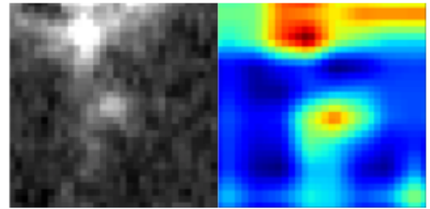
Fig. 13. Example of a misclassified OT (FN) by O'TRAIN. While the CNN focuses a fraction of its attention into the central part of the cutouts (where the OT is), most of its classification decision relies on the presence of a brighter source and a non-uniform background noise at the top of the cutouts.
