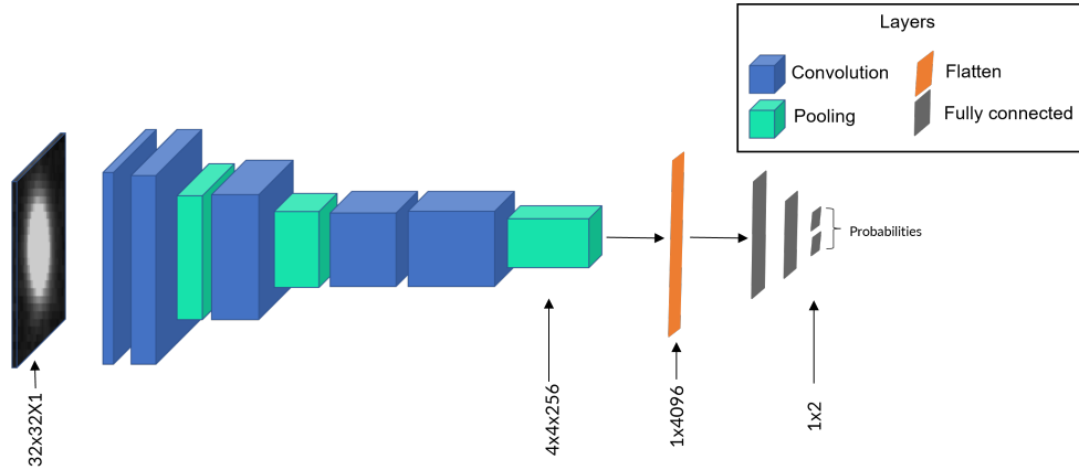
Fig. 1. Illustration of the O'TRAIN model architecture for performing the binary classification task: real or bogus transients.
