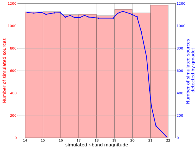
Fig. 4. Numbers of simulated point-like sources injected in the JAST images (red histogram) and retrieved by the GMADET transient detection pipeline (blue curve) as function of their simulated magnitudes. The source fluxes are computed from an arbitrarily chosen zero point magnitude value. The drop observed at magnitude r \sim 20.5 in the blue curve shows the point at which the sources are close to the detection threshold used in the GMADET pipeline.
