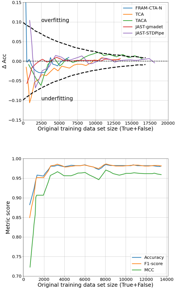
Fig. 11. Top: Evolution of \Delta\text{Acc} between the batch and the validation data sets as function of the size of the initial training data set after 25 epochs. This visualisation allows to quickly identify if the CNN algorithm is in an over(under)fitting regime (outliers of the dashed lines). Bottom: Evolution of three metrics: accuracy, F1 -score and MCC as a function of the training data set size (JAST-GMADET).
