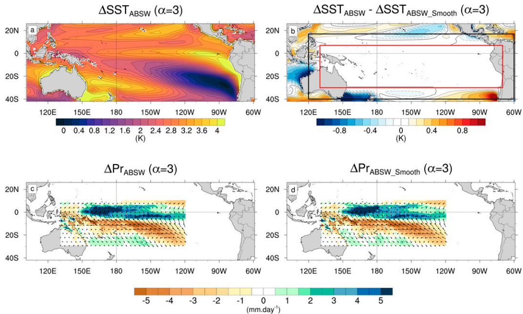
FIG. A1. (top) DJF climatology (in ^{\circ}\text{C} ) of (a) \Delta\text{SST}_{\text{ABSW}}(\alpha=3) and (b) difference between \Delta\text{SST}_{\text{ABSW}} and \Delta\text{SST}_{\text{ABSW\_Smooth}} . The red box represents the area where \Delta\text{SST}_{\text{ABSW\_Smooth}} = \Delta\text{SST}_{\text{ABSW}} (for \alpha = 3 ), the space between the black and red boxes represents the area where the smoothing is applied from \Delta\text{SST}_{\text{ABSW}} (for \alpha = 3 ) to \Delta\text{SST}_{\text{ABSW}} (for \alpha = 1 ), and outside of the black box \Delta\text{SST}_{\text{ABSW\_Smooth}} = \Delta\text{SST}_{\text{ABSW}} (for \alpha = 1 ). (bottom) Averaged DJF precipitation (shading; in \text{mm day}^{-1} ) and surface wind (vectors; in \text{m s}^{-1} ) changes (relative to CTRL simulation) in (c) ABSW (for \alpha = 3 ) and in (d) ABSW_Smooth.
