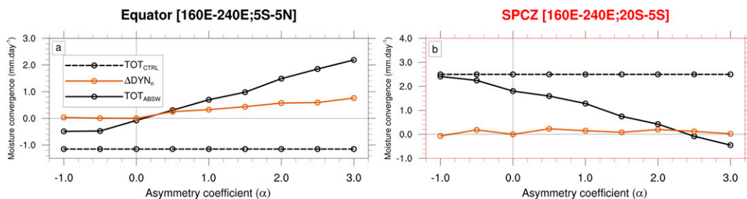
FIG. 7. Moisture convergence. Average DJF moisture convergence (in \text{mm}\cdot\text{day}^{-1} ) in ABSW (black thick lines), CTRL (black dashed lines), and dynamical contributions to the ABSW minus RELW moisture convergence change (brown) as a function of \alpha (a) in the equatorial box (black box in Fig. 5a) and (b) in the SPCZ box (red box in Fig. 5a).
