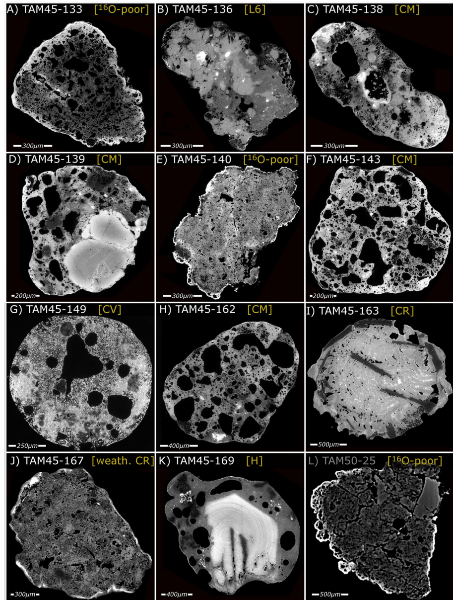
Figure 2. (A–K) Example \mu\text{CT} slices for each of the 11 micrometeorites analyzed in this study. (L) Also included is the anomalous ^{16}\text{O} -poor micrometeorite published in Suttle et al. (2020) TAM50-25. Parent body interpretations are also given for each particle (shown in yellow). Note some images are affected by ring artifacts centered on the rotational axis of the particle arising due to shifts in the output efficiency of individual detectors. These rings should be ignored as they are not a petrographic feature of the samples (Ketcham & Carlson, 2001).
