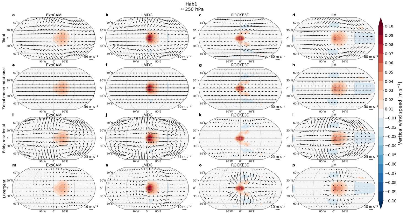
Figure 9. Helmholtz decomposition of the horizontal wind at 250 hPa in the Hab 1 case (quivers): (a)–(d) total wind, (e)–(h) zonal mean rotational component, and (m)–(p) divergent component. Note the different scaling of the eddy rotational and divergent components. Also shown is the upward wind velocity (shading, \text{m s}^{-1} ) with the 0.05 \text{ m s}^{-1} highlighted by a black contour. Note that for ExoCAM, only the pressure velocity ( \omega , \text{Pa s}^{-1} ) is available in the output, so the vertical velocity ( w , \text{m s}^{-1} ) is approximated as w = -\omega/\rho g , where \rho is air density and g is the acceleration due to gravity.
