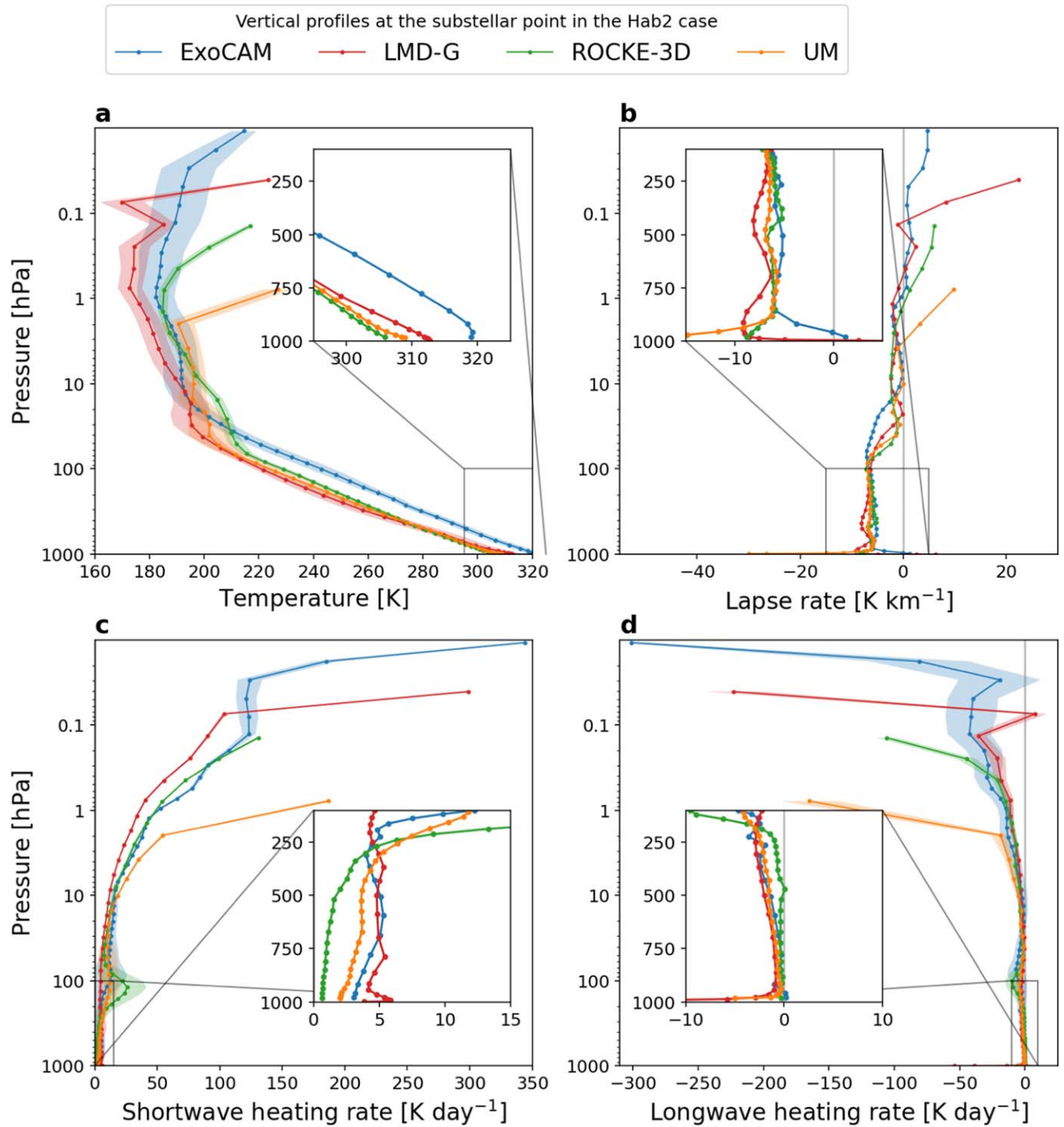
Figure 15. Hab 2 results: substellar vertical profiles of (a) air temperature (K), (b) lapse rate ( \text{K km}^{-1} ), (c) SW heating rate ( \text{K d}^{-1} ), and (d) LW heating rate ( \text{K d}^{-1} ). Time-mean values are shown by solid lines, the 1\sigma deviation is shown by shading.
