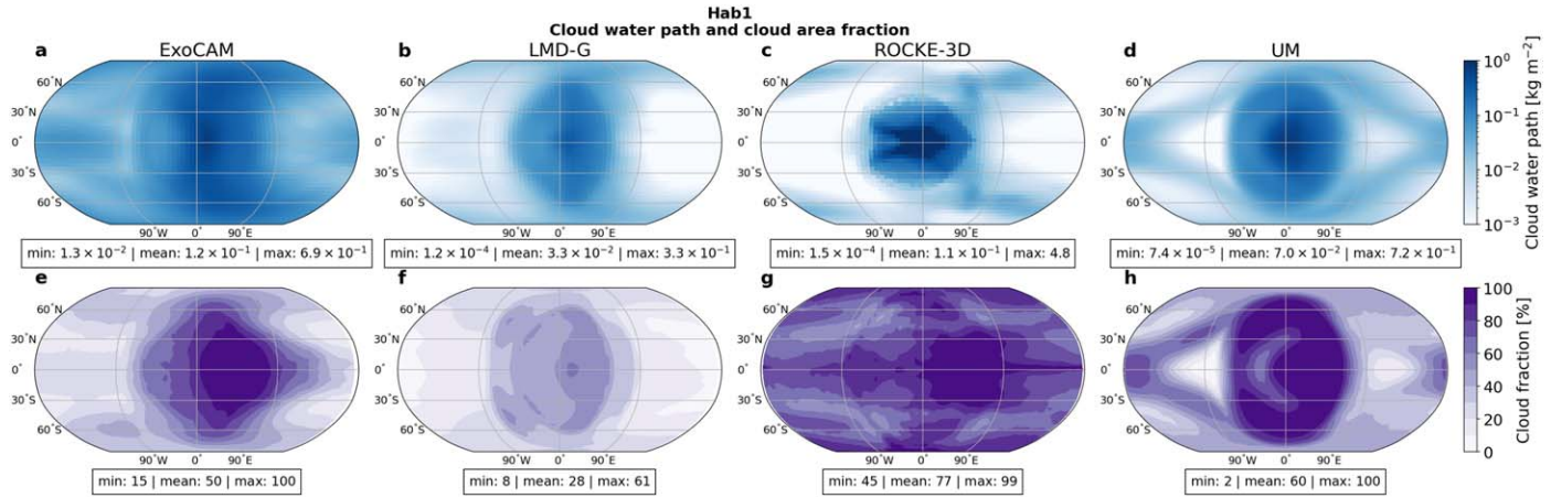
Figure 8. Hab 1 results: (a)–(d) cloud water path (vertically integrated cloud condensate content, \text{kg m}^{-2} ), and (e)–(h) cloud fraction (%).
