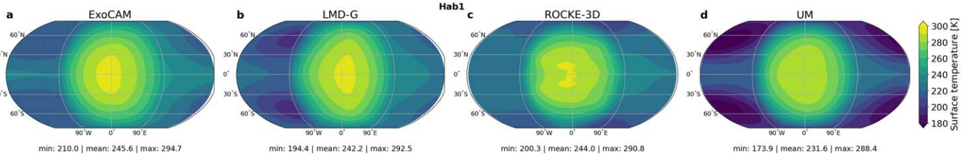
Figure 3. Hab 1 results: time-mean surface temperature (K) in (a) ExoCAM, (b) LMD-G, (c) ROCKE-3D, and (d) the UM.
