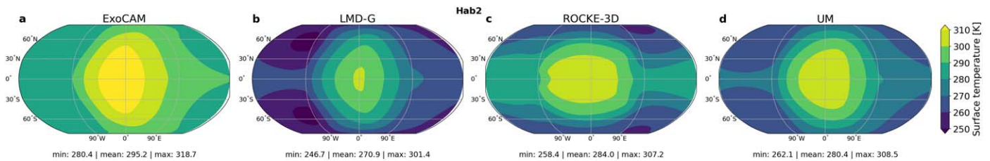
Figure 16. Hab 2 results: time-mean surface temperature (K) in (a) ExoCAM, (b) LMD-G, (c) ROCKE-3D, and (d) the UM.
