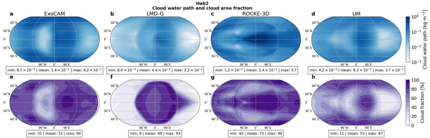
Figure 19. Hab 2 results: (a)–(d) cloud water path (vertically integrated cloud condensate content, \text{kg m}^{-2} ), and (e)–(h) cloud fraction (%).
