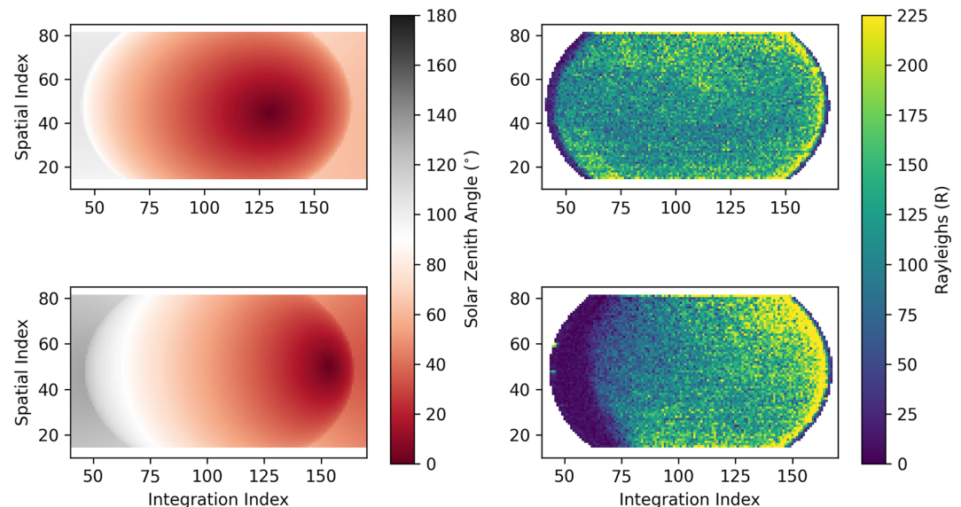
Figure 2. Solar zenith angles (left) and solar Lyman \alpha excited carbon monoxide Fourth Positive Group intensity (right) for the second swath (out of three) for OS-2 observations on 24 April 2021 (top row) and 18 June 2021 (bottom row).
