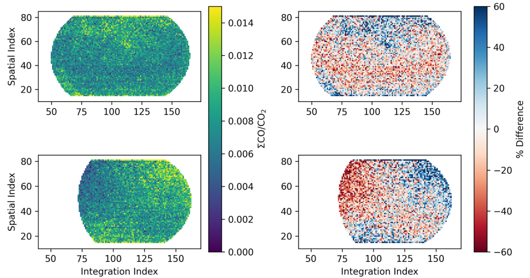
Figure 3. Retrieved \Sigma\text{CO}/\text{CO}_2 (left) and percent difference from swath averaged \Sigma\text{CO}/\text{CO}_2 (right) for the observations shown in Figure 2.
