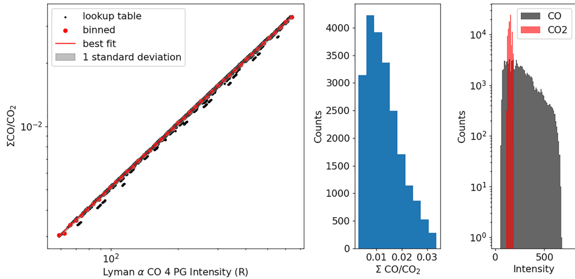
Figure 1. Left: Ratio of modeled carbon monoxide (CO) Fourth Positive Group column emission rates (Rayleighs) produced by CO as a function of \Sigma\text{CO}/\text{CO}_2 column density ratio. Model values are shown as black dots and correspond to an SZA of 0^\circ and EMA of 0^\circ . The scatter seen in the model ratios is due to variations in \text{N}_2 and Ar mixing ratios. Center: Histogram of lookup table \Sigma\text{CO}/\text{CO}_2 column density ratios. Right: Histogram of CO (gray) and \text{CO}_2 (red) lookup table intensities (Rayleighs) for SZA and EMA <35^\circ .
