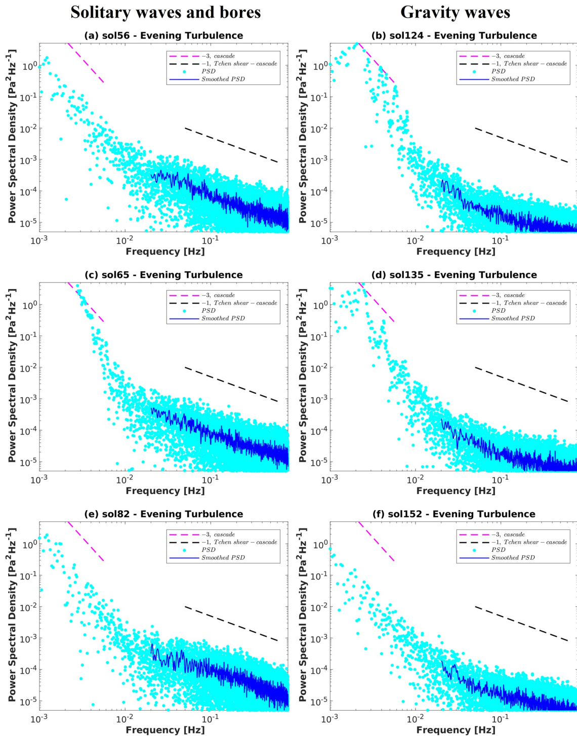
Figure 3. Turbulence spectra acquired for the days with and without solitary waves and bores (left panel, sol 65 with solitary wave and bores), and gravity waves (right panel, sol 124 and 135 with gravity waves). The sols are selected according to the gravity wave activity catalog acquired based on the InSight lander's pressure observations (Banfield et al., 2020).
