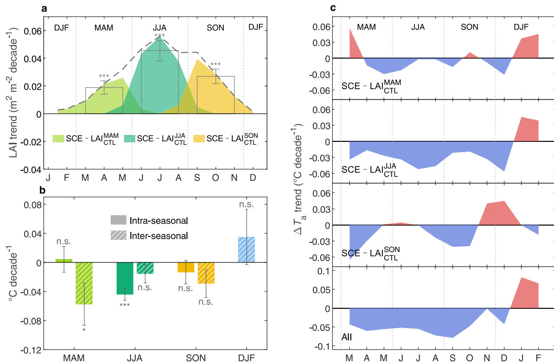
Fig. 1 Intra- and inter-seasonal temperature responses to leaf area index (LAI) changes. a Monthly trends (shadings) of Northern Hemisphere (NH) mean LAI during 1982–2014 used as input to the seasonal simulations. The dashed curve and transparent bars indicate trends of monthly LAI and seasonally aggregated LAI values, respectively. b Linear trends of T_a driven by LAI changes within the same season (intra-seasonal) and other growing seasons (inter-seasonal). Error bars in a , b indicate uncertainty ranges [ 1 - \text{standard deviation (SD)} ]. c Monthly trends of LAI-induced air temperature changes ( \Delta T_a ), with red and blue shadings representing positive and negative trends, respectively. The bottom panel shows the overall \Delta T_a trends induced by LAI changes in all growing seasons, calculated as the sum of \Delta T_a trends from the three seasonal runs shown separately in the above panels. *** p < 0.01 ; ** p < 0.05 ; * p < 0.1 ; n.s., p > 0.1 . MAM March–April–May, JJA June–July–August, SON September–October–November, DJF December–January–February.
