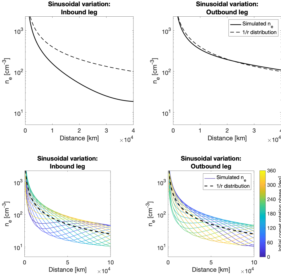
Fig. 6. The along-track observed ionospheric density for the case of a sinusoidally varying outgassing rate. A 1/r -distribution is included for comparison (dashed line). Note the significant difference between the profiles on the inbound and the outbound leg.
