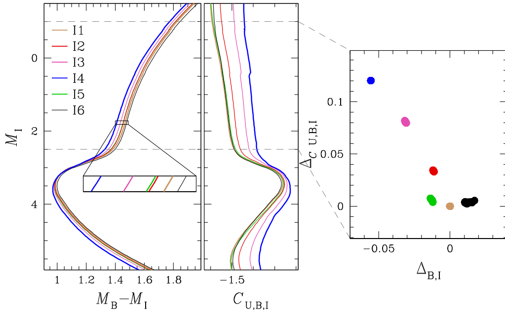
Figure 9. The six coloured lines plotted in the left-hand and middle panels represent the isochrones I1–I6 (see Table 1 for details on their chemical compositions). The \Delta_{C_{U,B,I}} versus \Delta_{B,I} ChM of the RGB stars between the dashed horizontal lines is plotted in the right-hand panel.
