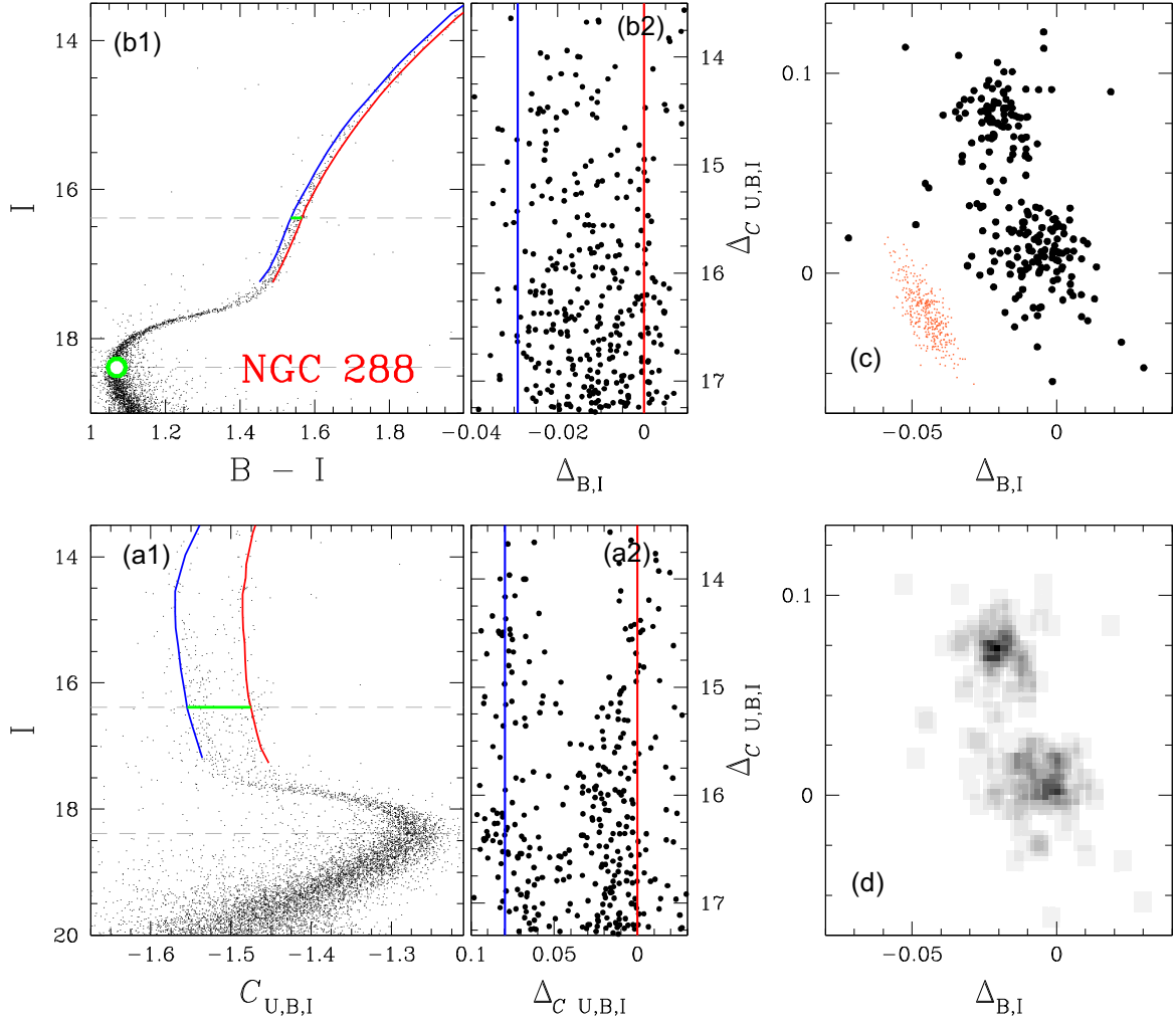
Figure 7. This figure illustrates the procedure to derive the \Delta_{C_{U,B,I}} versus \Delta_{B,I} ChM for the prototypical cluster NGC 288. Panels (a1) and (b1) show the I versus C_{U,B,I} pseudo-CMD and I versus B - I CMD of NGC 288. The green circle in panel (b1) marks the MS turnoff, whereas the two horizontal dotted lines in panels (a1) and (b1) are placed at the magnitude level of the MS turnoff and 2.0 I mag above it. The blue and red lines mark the boundaries of the RGB, while the green segments in the panels (a1) and (b1) indicate the B - I colour and the C_{U,B,I} pseudo-colour separation between the two lines at 2.0 I mag above the MS turnoff. The ‘verticalized’ I versus \Delta_{C_{U,B,I}} and I versus \Delta_{B,I} diagrams for RGB stars are plotted in panels (a2) and (b2), respectively, where the red and blue vertical lines correspond to the RGB boundaries in panels (a1) and (b1) that translate into vertical lines in panel (a2) and (b2). The RGB stars used to construct the ChM in panel (c) are represented in panels (a2) and (b2), where \Delta_{C_{U,B,I}} and \Delta_{B,I} are plotted against I . Panel (d) shows the Hess diagram for stars in panel (c).
