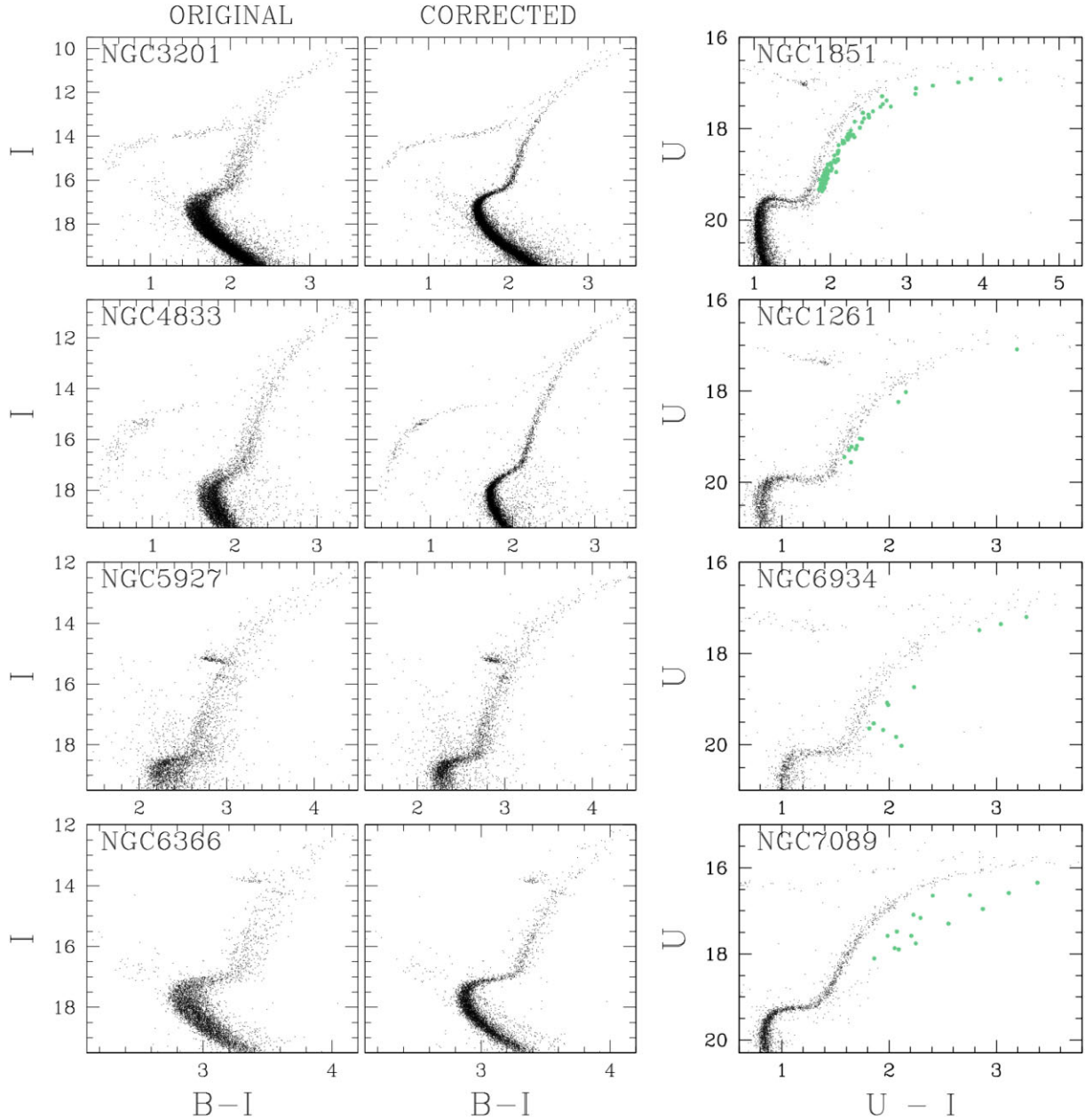
Figure 6. Comparison of the original I versus B-I CMDs of NGC 3201, NGC 4833, NGC 5927, and NGC 6366 (left-hand panels) with the CMDs corrected for differential reddening (middle panels). The right-hand panels show the U versus U-I CMD of the Type II GCs NGC 1851, NGC 1261, NGC 6934, and NGC 7089. Red RGB stars are coloured aqua.
