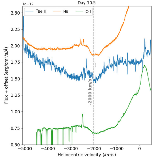
Figure 8. {}^7\text{Be} , \text{H}\delta , and \text{O I} triplet at 777.19, 777.41, and 777.54 nm spectra at day 10.5 plotted on a common velocity scale. The \text{O I} triplet is not resolved though, with a separation of 133 \text{ km s}^{-1} , and the \text{O I} 777.5388 nm wavelength is used for the zero velocity in the plot. Note that the absorption of \text{O I} is affected on the left by the emission line of \text{Fe II} (73) at 771.2 nm. No other metal elements are detected to check the common absorption system. The narrow absorption features present in the \text{O I} spectrum are the telluric lines of the molecular \text{O}_2 A band.
