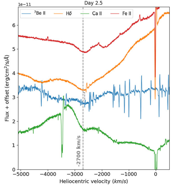
Figure 7. As the previous figure for day 2.5. We note the enhancement of the emission of the \text{H I} 388.905 nm line falling in the middle of the \text{Ca II} K absorption.
