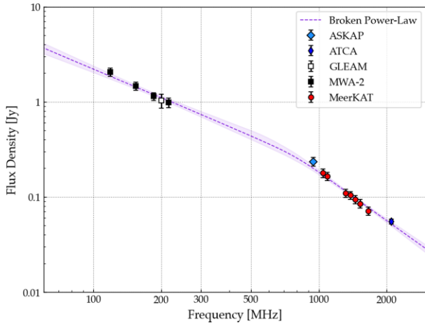
Figure 14. Spectral energy distribution (SED) for the complex tailed radio galaxy to the north-west of Abell 3266 (Source RG2; shown in Fig. 6). Our new ASKAP and ATCA measurements are shown as blue diamonds, in-band spectral measurements from the MeerKAT GCLS data are shown in red, and datapoints from the MWA from Duchesne et al. (2022) are shown as squares. Our best-fitting broken power-law spectrum is shown by the dashed violet line; the shaded region denotes the 1\sigma uncertainty.
