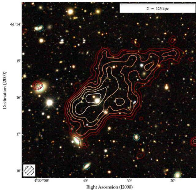
Figure 6. Radio-on-optical overlay of the ultra-steep spectrum fossil radio galaxy to the NW of Abell 3266 (source ‘D2’ in Fig. 1). Contours show the 943-MHz ASKAP surface brightness at 15-arcsec resolution, starting at 3\sigma and scaling by a factor of \sqrt{2} . The colourmap shows an optical RGB image from DES, as per Fig. 1. Dashed cyan circles denote cluster-member galaxies identified by Dehghan et al. (2017). The proposed host for this diffuse radio source is the cluster-member galaxy at the SE tip of the emission.
