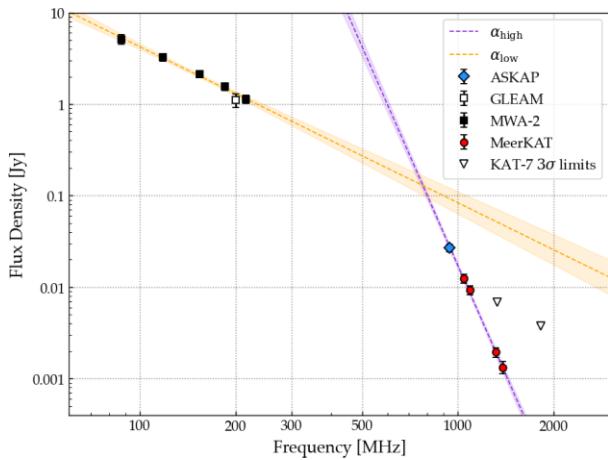
Figure 7. Spectral energy distribution (SED) for the ultrasteep spectrum fossil to the NW of Abell 3266 (Source D2; shown in Fig. 6). Our new ASKAP measurement is shown by the blue diamond; datapoints from the MWA (Duchesne et al. 2022) are shown as squares. Open triangles denote 3\sigma upper limits from KAT-7. In-band spectral measurements from the MeerKAT GCLS data (where the source was detectable above 3\sigma ) are shown in red. The spectral index is extremely steep, approximated by a power-law fit of \alpha_{\text{low}} = -1.70 \pm 0.14 between 88 and 216 MHz and \alpha_{\text{high}} = -7.92 \pm 0.30 between 943 and 1312 MHz. These fits are shown as dashed lines, with the shaded region denoting the 1\sigma uncertainty.
