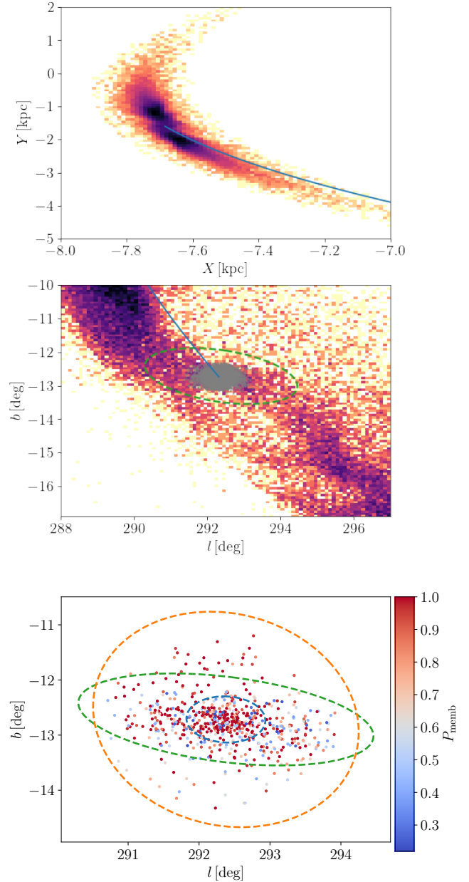
Fig. 1. Results of the simulation compared to the distribution of cluster members. Top and middle: ( X , Y ) and ( l , b ) distribution of the simulated escaping stars of the cluster. The colours correspond to the density of points, and the blue line indicates the orbit integrated backwards. In grey, we plot the stars which are still bounded to the cluster (energy < 0 ). Bottom: ( l , b ) distribution of the cluster members coloured by the probability of membership. The three ellipses correspond to the three Gaussian components obtained by our GMM fit in Sect. 2.2, corresponding to the core (blue), the tidal tail (green), and the halo (orange). The tidal tail ellipse is also plotted in the middle panel for comparison.
