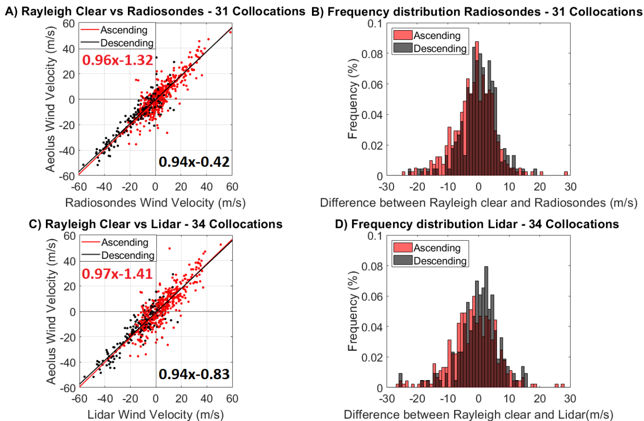
335 Figure 4. a) The Aeolus winds versus the radiosonde measurements made during all the campaigns. b) Frequency distribution of the difference between Aeolus and radiosonde wind speeds for the same data set. Red represents measurements of an ascending orbit, while black represents measurements of a descending orbit. c) The L2B Rayleigh clear winds versus the lidar measurements made during all the campaigns. d) Frequency distribution of the difference between Aeolus and lidar wind speeds for the same data set. Red represents measurements of an ascending orbit, while black represents measurements of a descending orbit.
