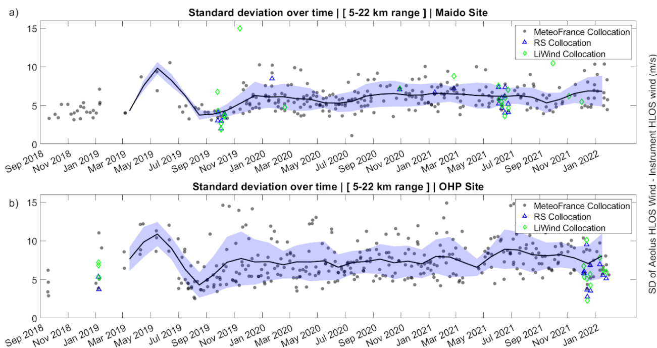
Figure 6. Standard deviation of the difference between Aeolus Rayleigh clear HLOS wind and Météo-France Radiosonde HLOS wind, over time a) at the Maido Observatory b) at the Haute Provence Observatory. The Météo-France data were downsampled to Aeolus vertical resolution and projected to the HLOS of Aeolus. For radiosonde and ground-based lidar collocations, the cal/val punctual collocations are reported in the figure in blue and green markings.
