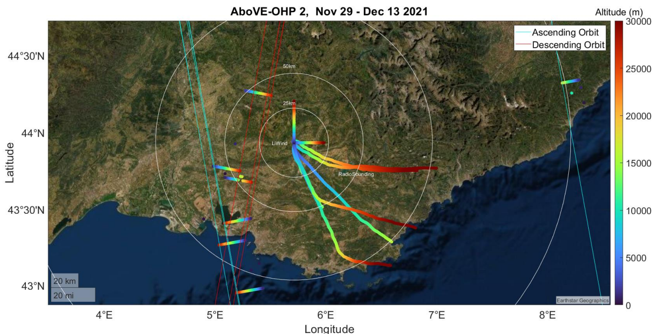
270 Figure 2. AboVE-OHP 2 Campaign overview with ascending and descending overpasses in cyan and red. The colored trajectories represent the ascending phase of the radiosondes, with their altitude shown through a colormap. Credit: base map sources are Earthstar Geographics.
