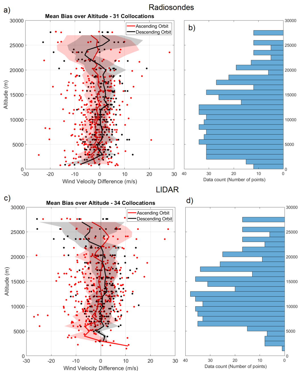
300 Figure 3. a) The Aeolus minus the radiosonde HLOS wind difference made during all AboVE campaigns over each altitude bin. b) The number of data samples over each altitude bin for the radiosonde comparison. c) The Aeolus minus the lidar HLOS wind difference made during all the campaigns over each altitude bin. d) The number of data samples over each altitude bin for the Lidar comparison. Red represents measurements of an ascending orbit, while black represents measurements of a descending orbit. The lines represent the average bias of each bin altitude, and the shading is the standard deviation of the bias in each range bin.
