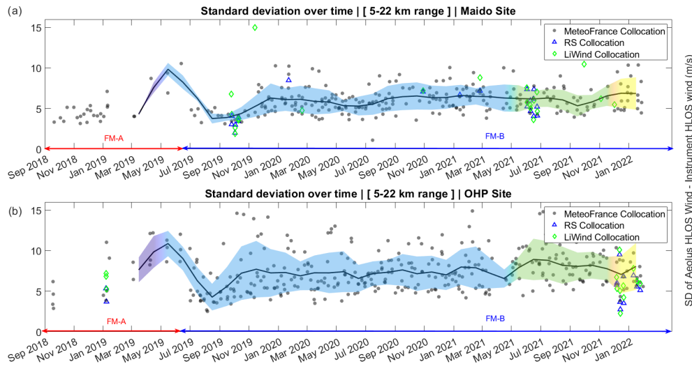
Figure 6. Standard deviation of the difference between Aeolus Rayleigh clear HLOS wind and Météo-France Radiosonde HLOS wind over time (a) at the Maito observatory and (b) at the Observatoire de Haute-Provence. The Météo-France data were downsampled to Aeolus vertical resolution and projected to the HLOS of Aeolus. For radiosonde and ground-based lidar collocations, the cal/val punctual collocations are reported in the figure in blue and green markings. The black line represents the average value, and the shading represents its standard deviation. The colors are relative to the four baselines used: 2B02 (violet), 2B11 (blue), 2B12 (green), and 2B13 (yellow), in that order.
