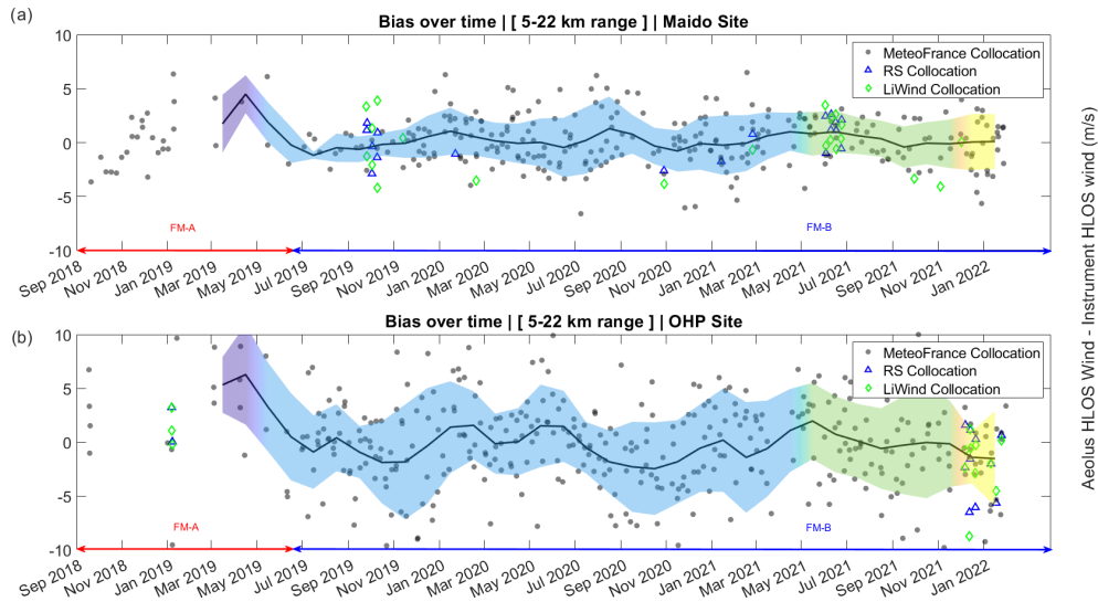
Figure 7. Bias between Aeolus Rayleigh clear HLOS wind and Météo-France radiosonde HLOS wind over time (a) at the Maido observatory and (b) at the Observatoire de Haute-Provence. The Météo-France data were downsampled to Aeolus vertical resolution and projected to the HLOS of Aeolus. For radiosonde and ground-based lidar collocations, the cal/val punctual collocations are reported in the figure in blue and green markings. The black line represents the average value, and the shading represents its standard deviation. The colors are relative to the four baselines used: 2B02 (violet), 2B11 (blue), 2B12 (green), and 2B13 (yellow), in that order.
