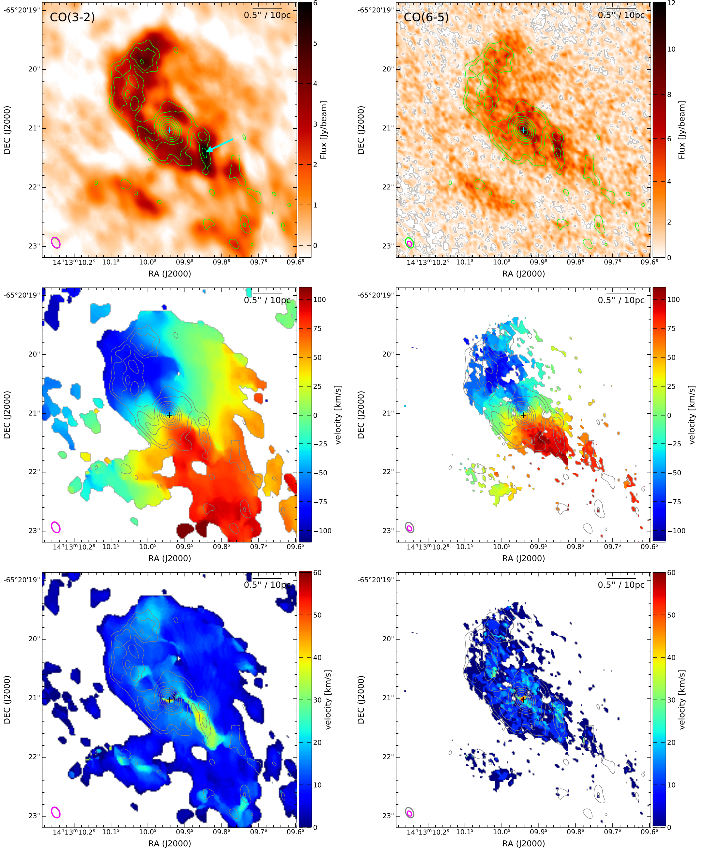
Fig. 2. CO(3–2) ( v_{\text{rest}} = 346 GHz, \lambda_{\text{rest}} = 867 \mu\text{m} , left panels ) and CO(6–5) ( v_{\text{rest}} = 691 GHz, \lambda_{\text{rest}} = 434 \mu\text{m} , right panels ) moment maps. Top row: the total integrated line emission (moment 0) maps are shown; in the middle row , the velocity (moment 1) maps are displayed; the bottom row shows the velocity dispersion (moment 2). The green/grey contours in all panels are for the 345 GHz continuum as in Fig. 1. The cyan arrow in the top left panel marks the ridge-like structure discussed in the text.
