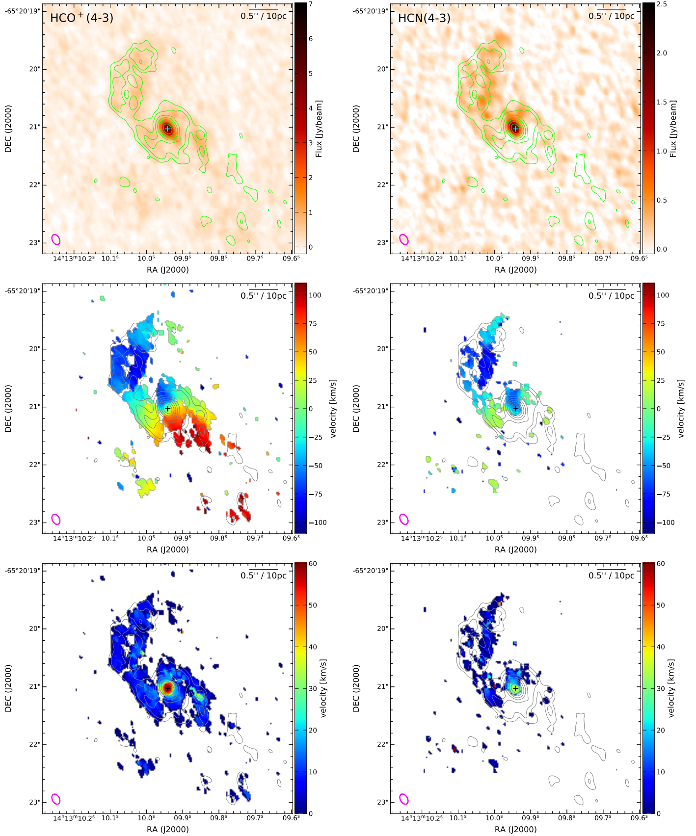
Fig. 3. HCO + (4–3) ( \nu_{\text{rest}} = 357 GHz, left panels ) and HCN(4–3) ( \nu_{\text{rest}} = 355 GHz, right panels ) moment maps. Top row : the total integrated line emission (moment 0) maps are shown; in the middle row , the velocity (moment 1) maps are displayed; the bottom row shows the velocity dispersion (moment 2). The green/grey contours in all panels are for the 345 GHz continuum as in Fig. 1. For HCN(4–3), only the velocity range from -300 to +15 km s -1 is covered by the observations, so that the south-western, redshifted part of the emission is missing (see Sect. 2).
