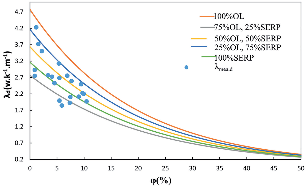
Figure10. Thermal conductivity calculation from the geometric mean model as a function of porosity and serpentinization degree. The porosity thermal conductivity trend established in our study is shown with blue circle.
